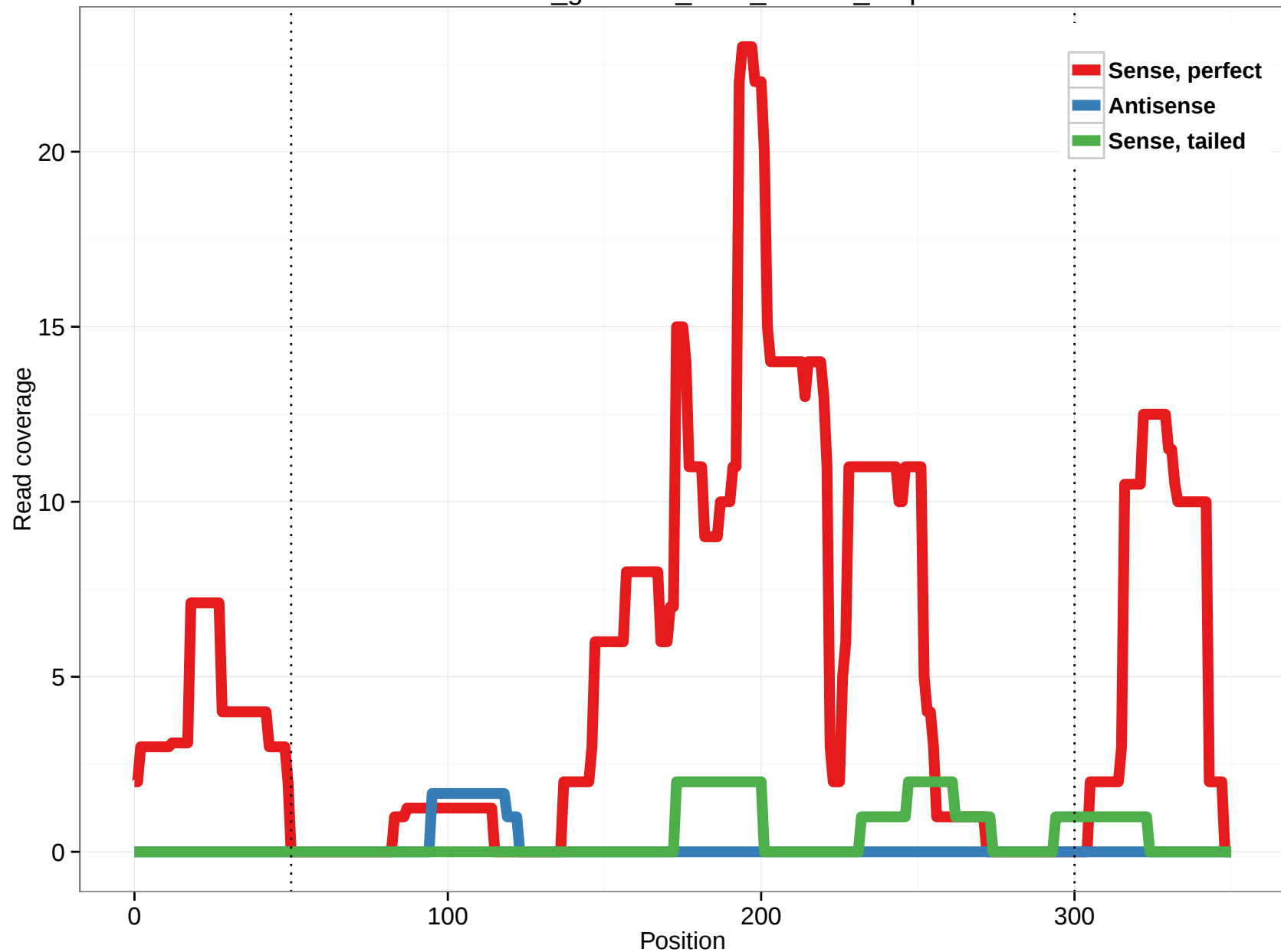
rheMac3_genscan_chrX_235.12_5.3p
