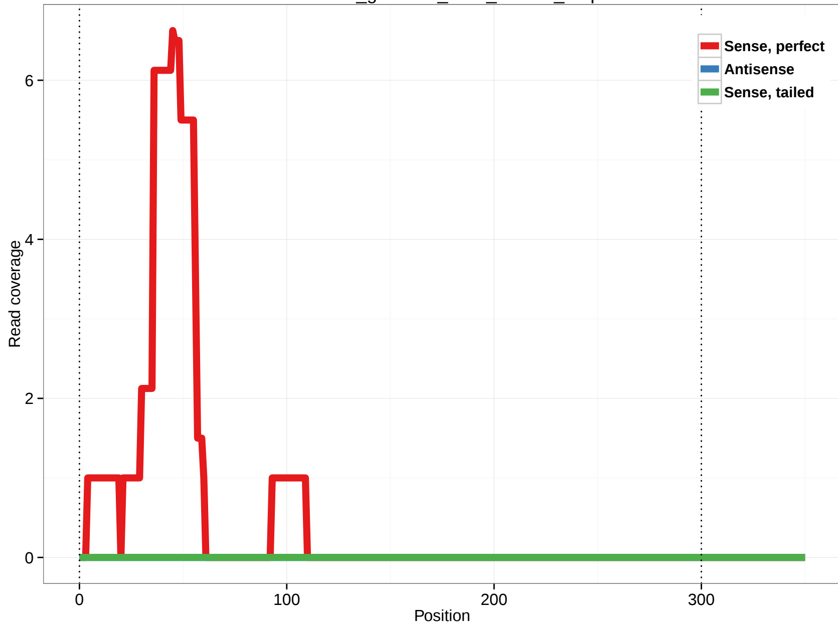
rheMac3_genscan_chrX_235.10_3.3p
