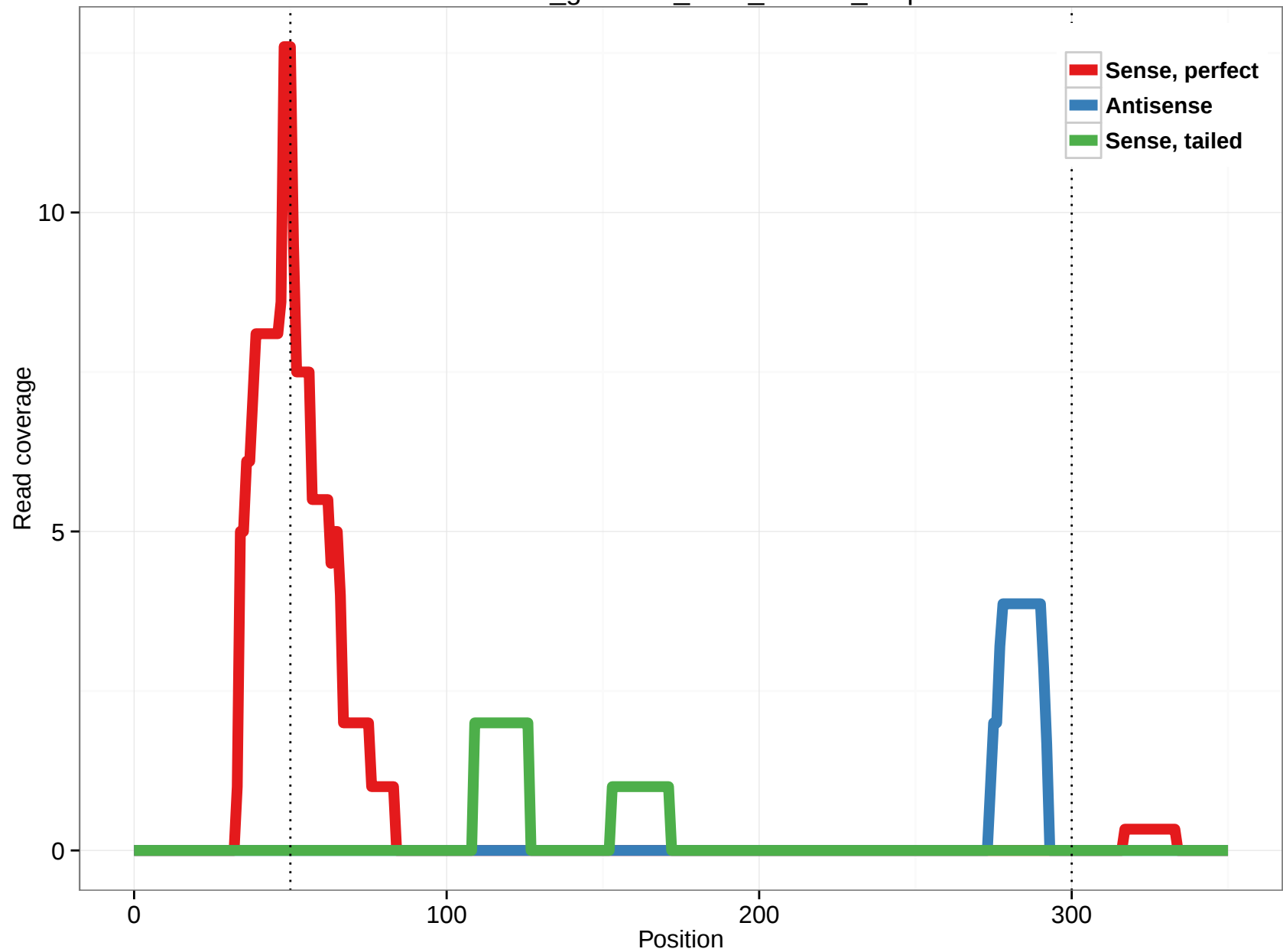
rheMac3_genscan_chrX_226.17_0.3p
