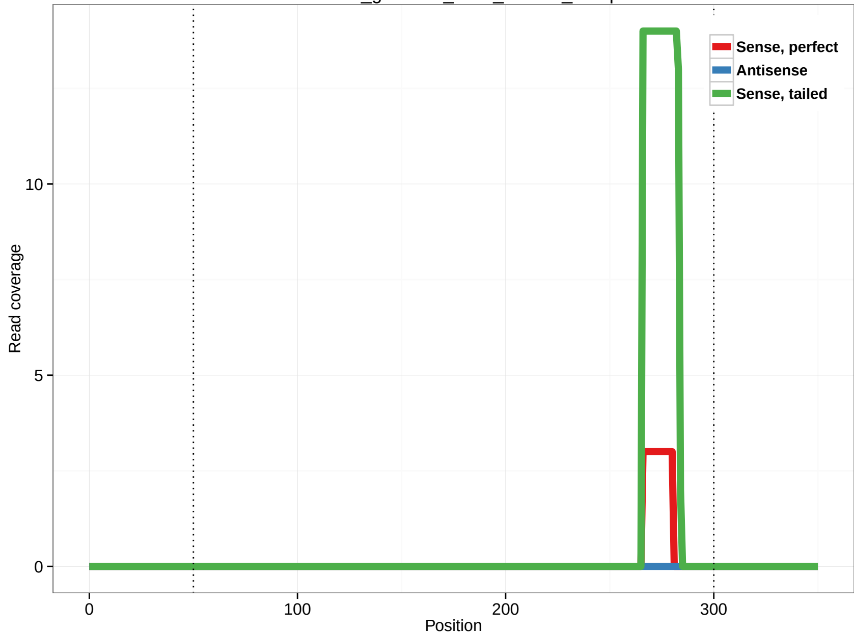
rheMac3_genscan_chrX_225.13_17.5p
