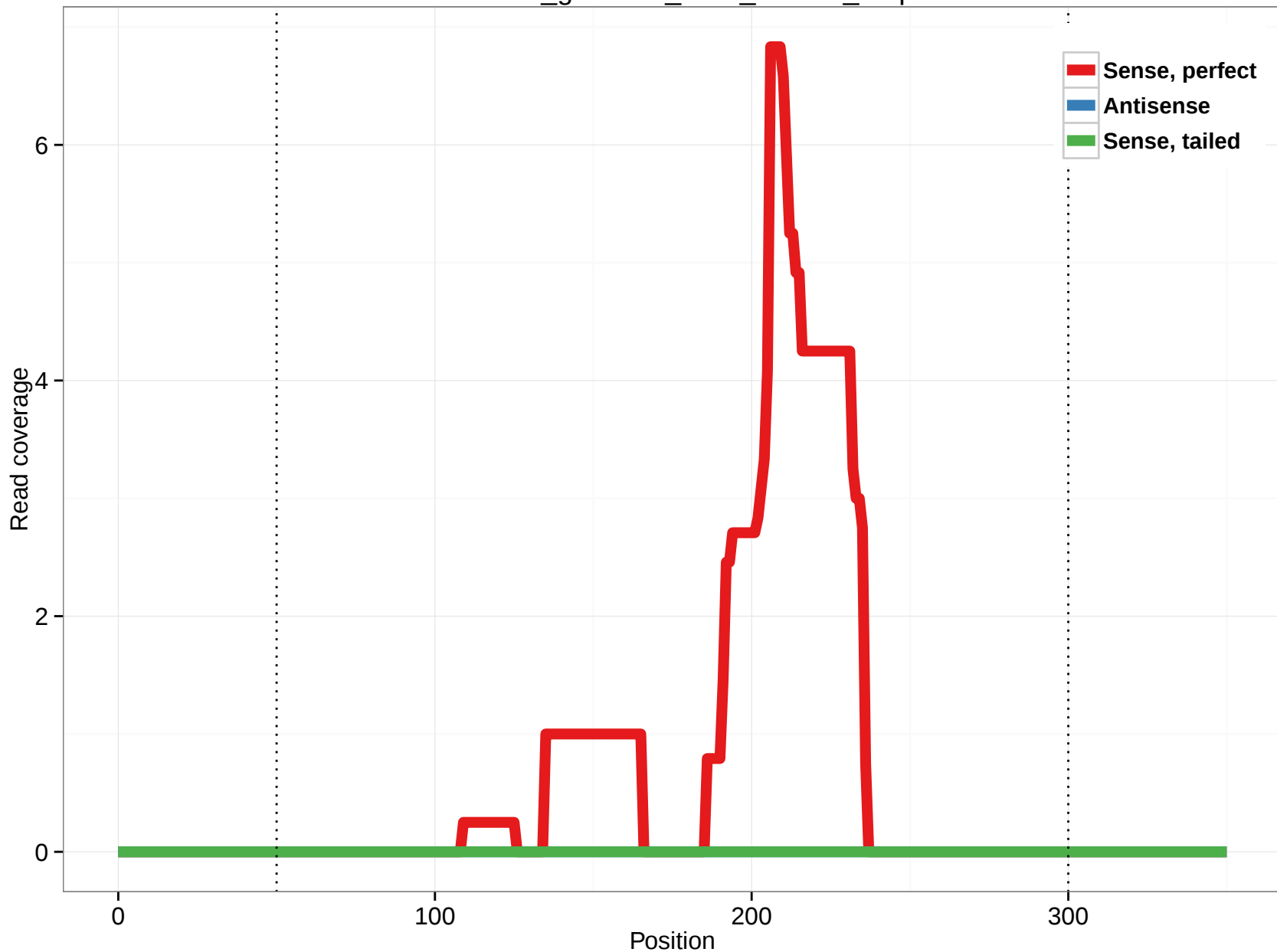
rheMac3_genscan_chrX_213.36_1.3p
