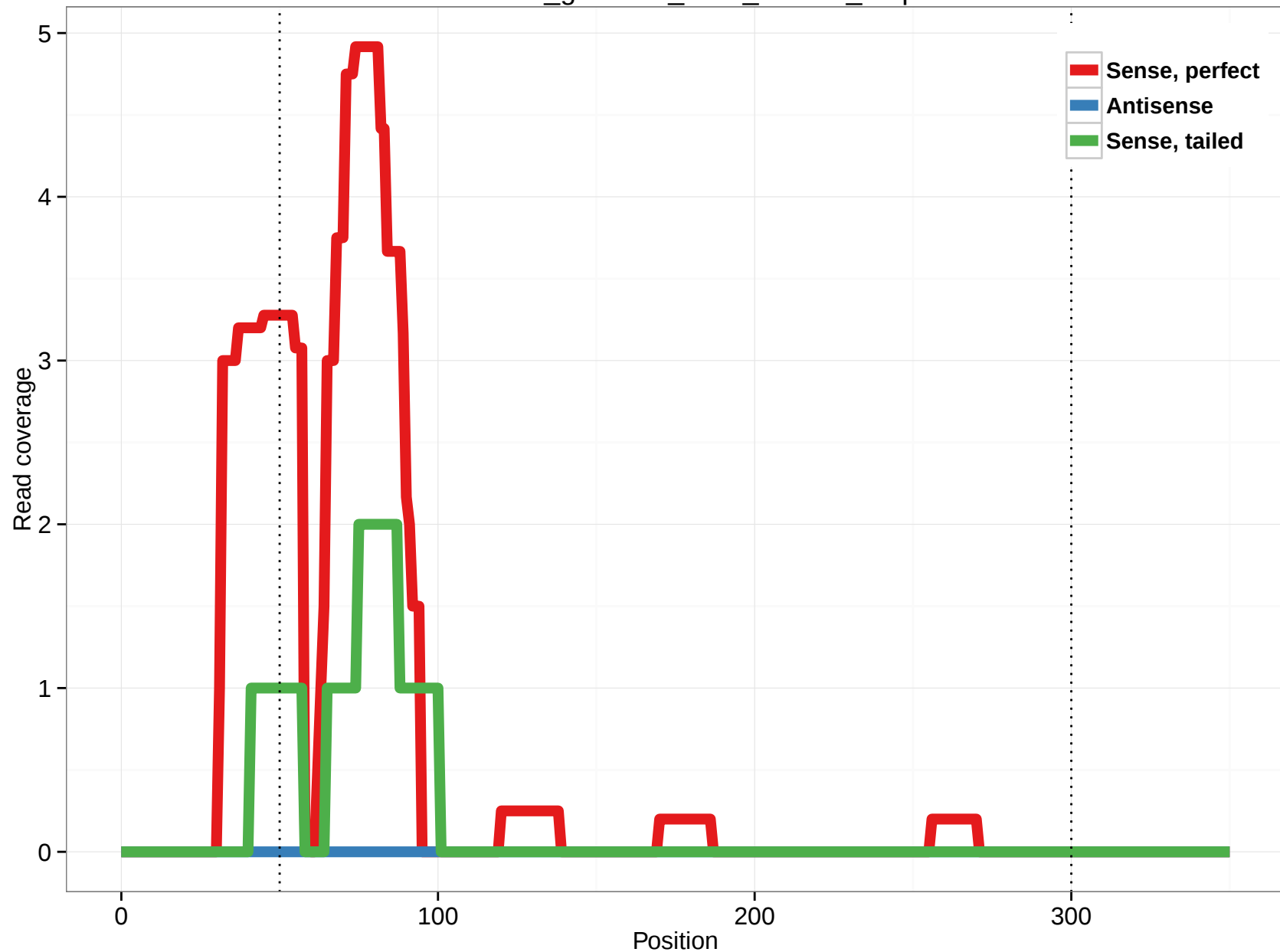
rheMac3_genscan_chrX_209.10_0.5p
