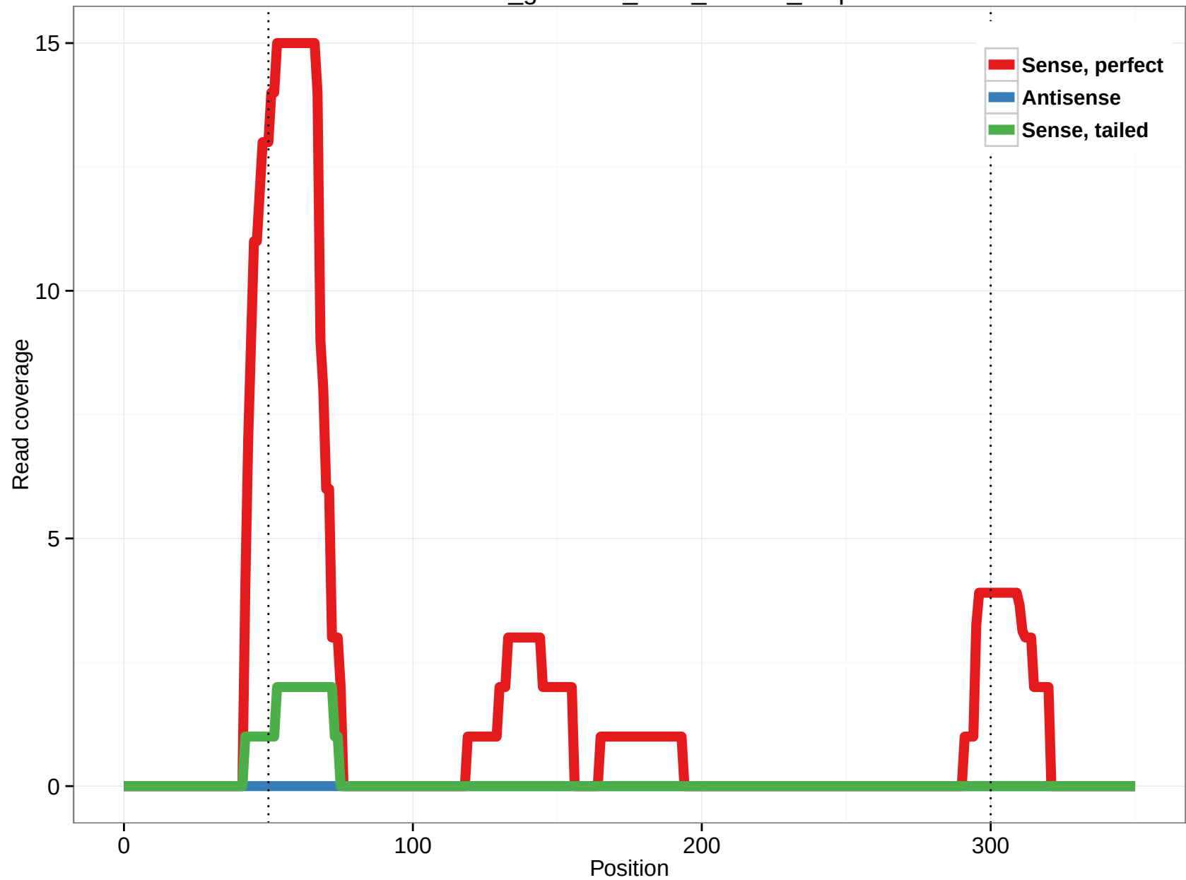
rheMac3_genscan_chrX_206.12_5.3p
