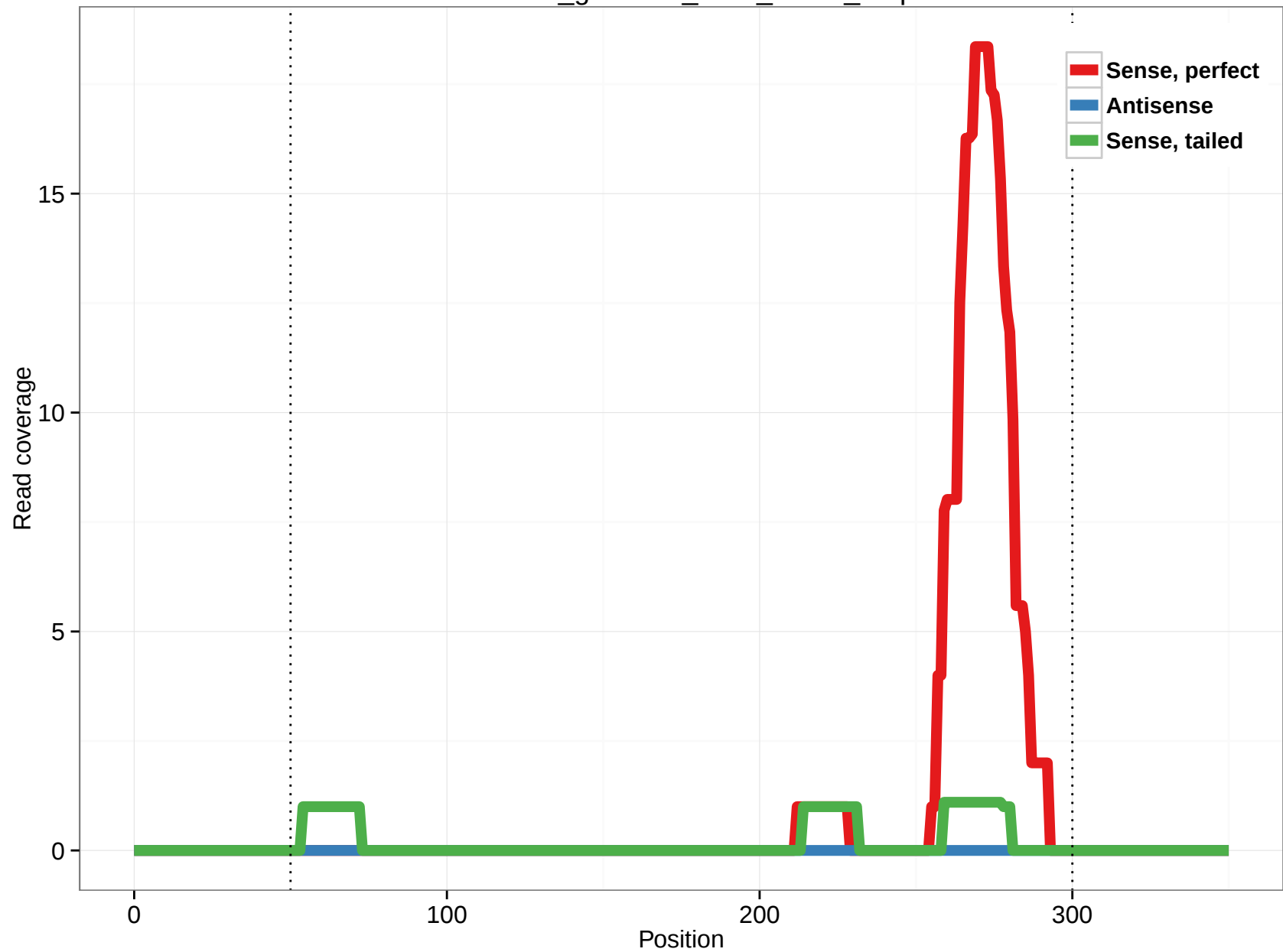
rheMac3_genscan_chrX_193.9_6.3p
