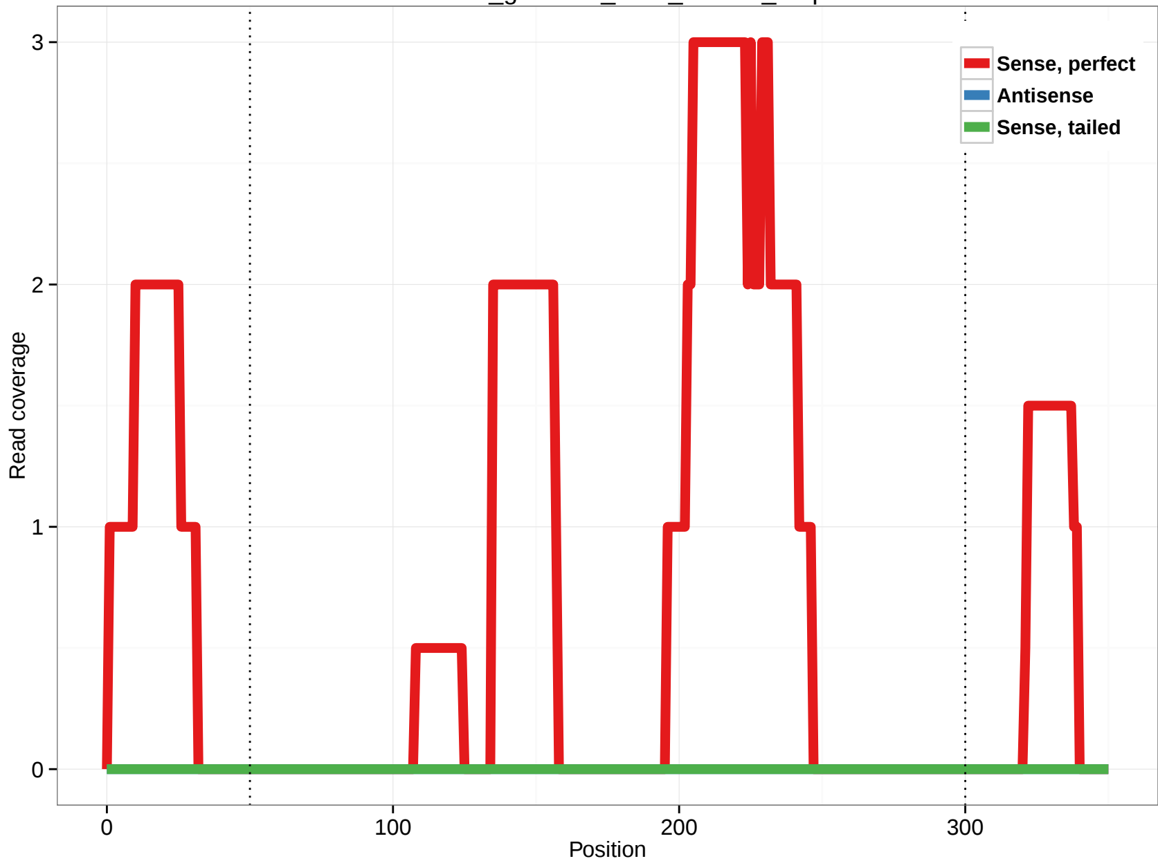
rheMac3_genscan_chrX_193.10_2.5p
