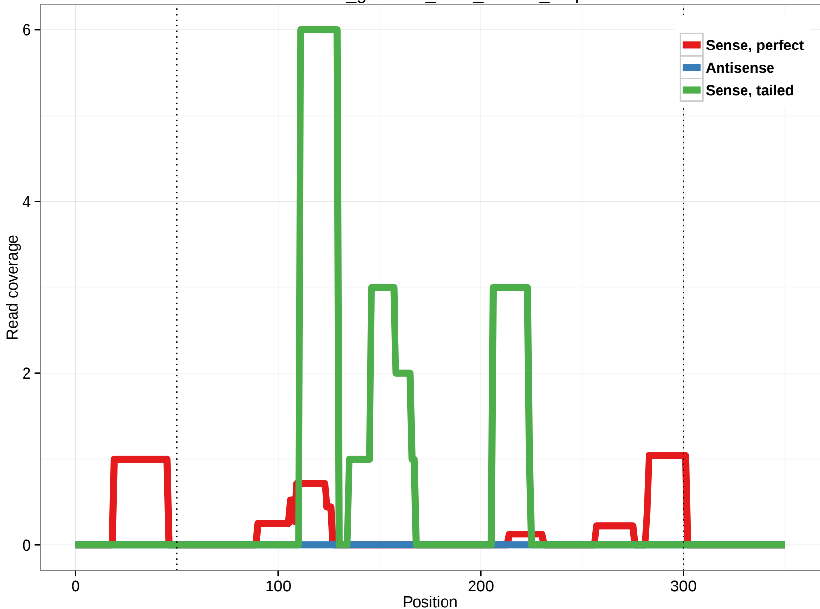
rheMac3_genscan_chrX_180.17_6.5p
