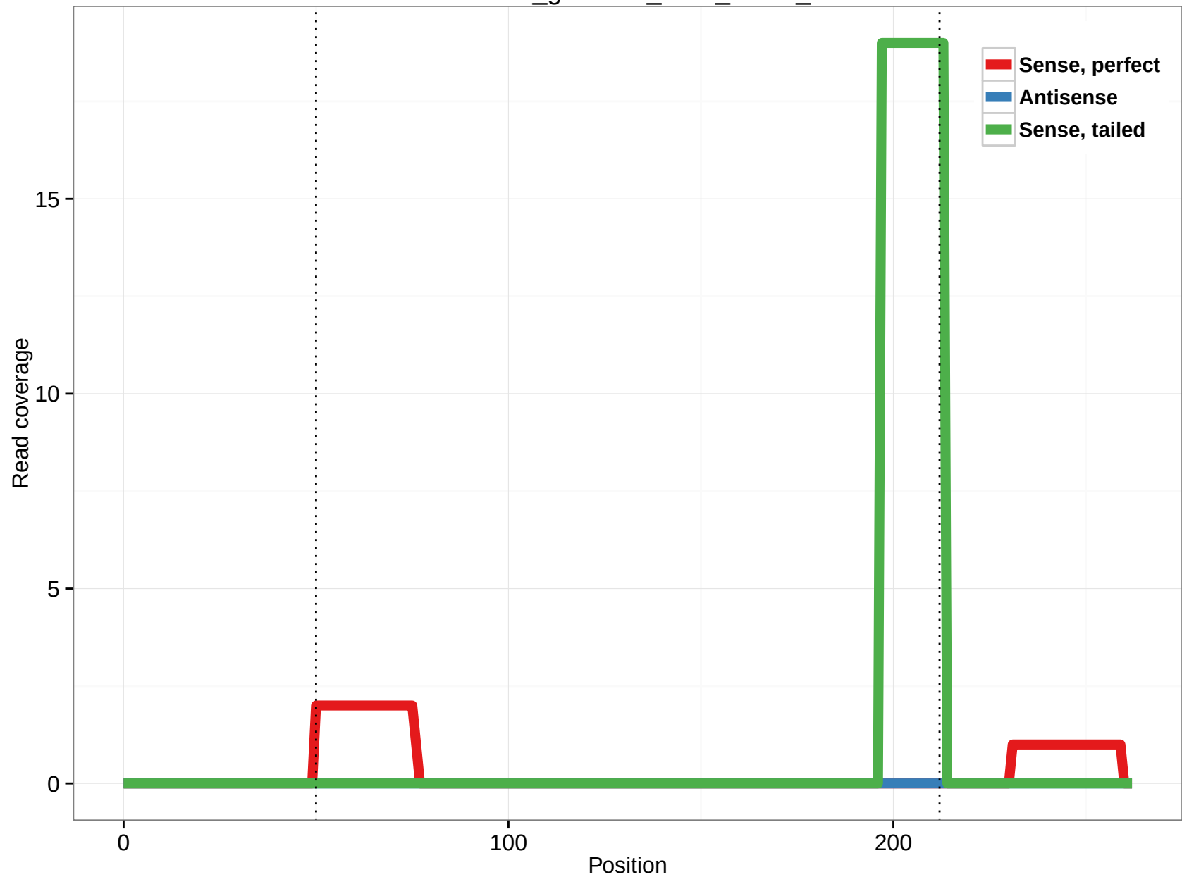
rheMac3_genscan_chrX_160.6_2
