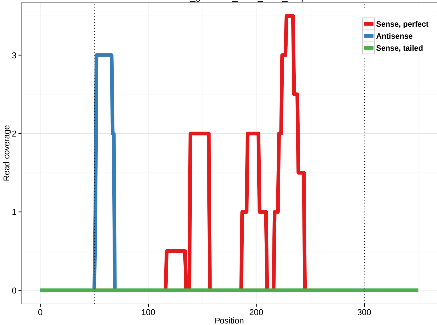
rheMac3_genscan_chrX_16.9_2.5p
