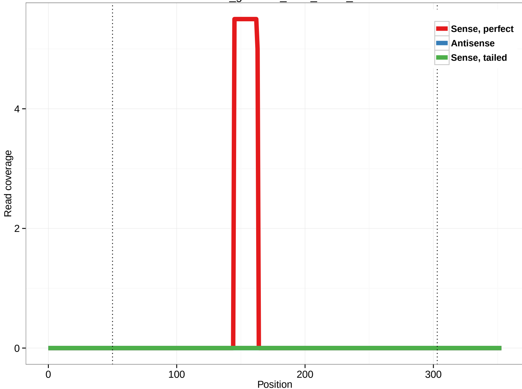
rheMac3_genscan_chrX_16.27_19
