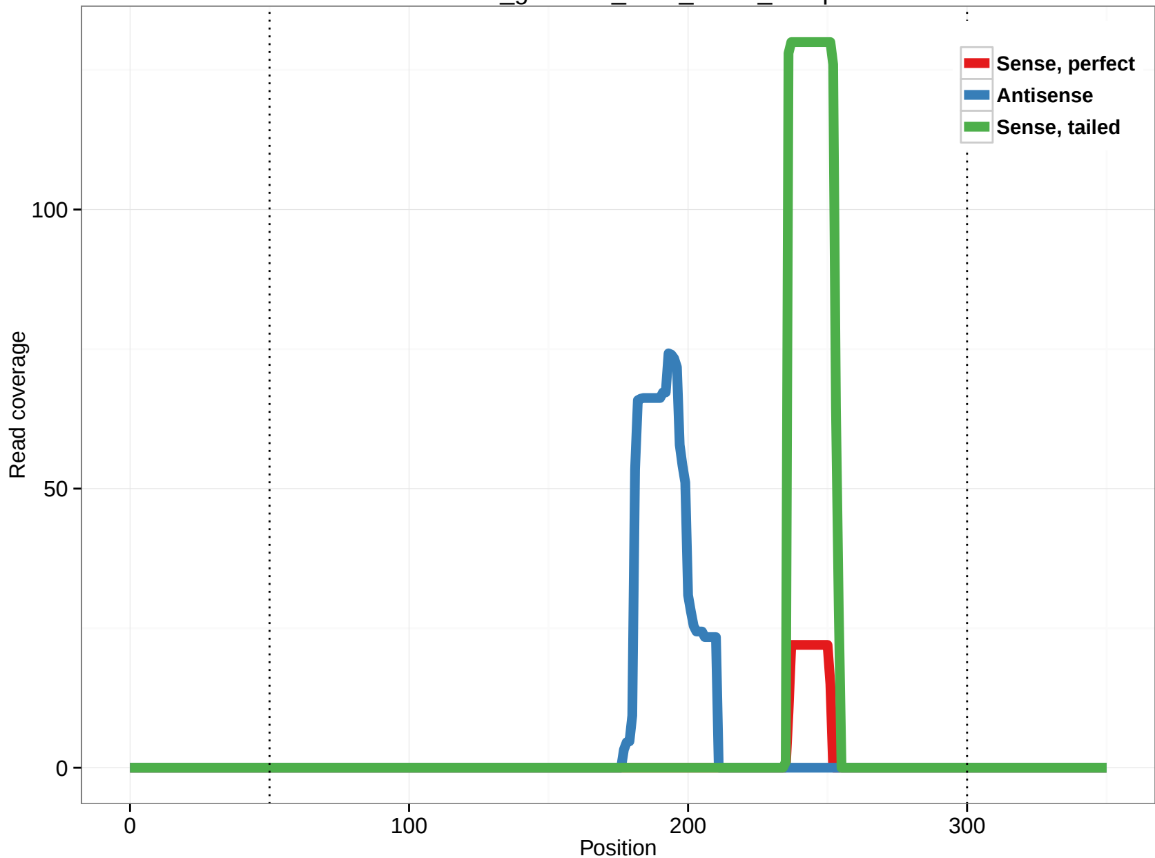
rheMac3_genscan_chrX_16.18_26.3p
