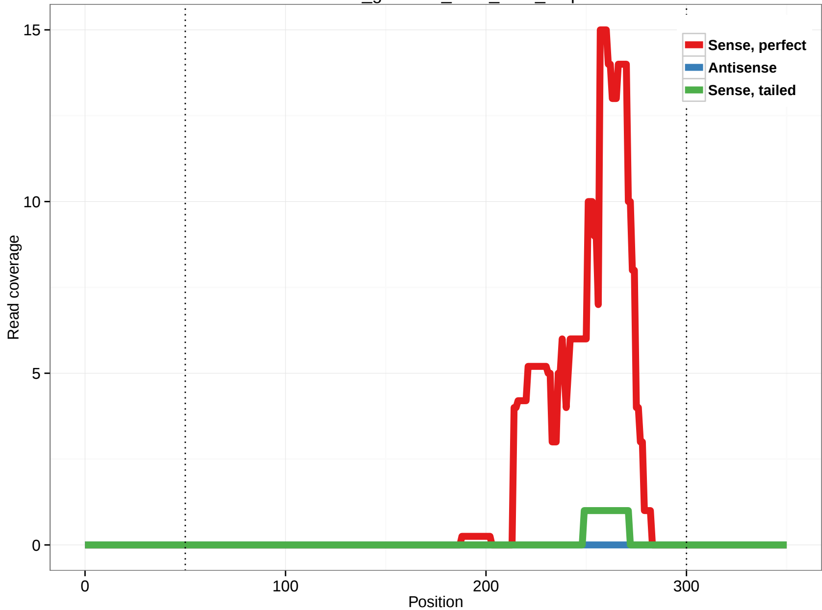
rheMac3_genscan_chrX_14.6_9.3p
