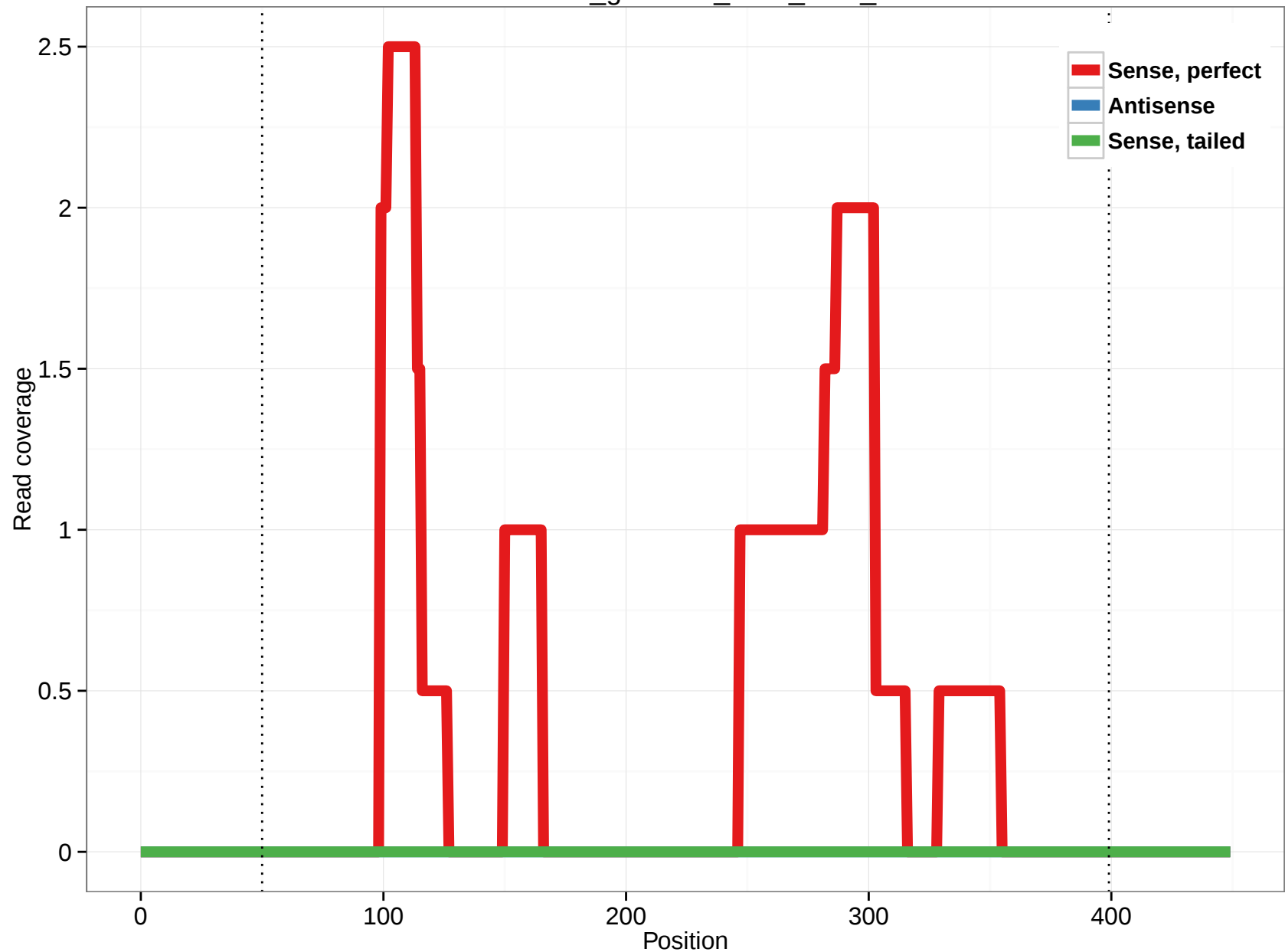
rheMac3_genscan_chrX_11.6_2
