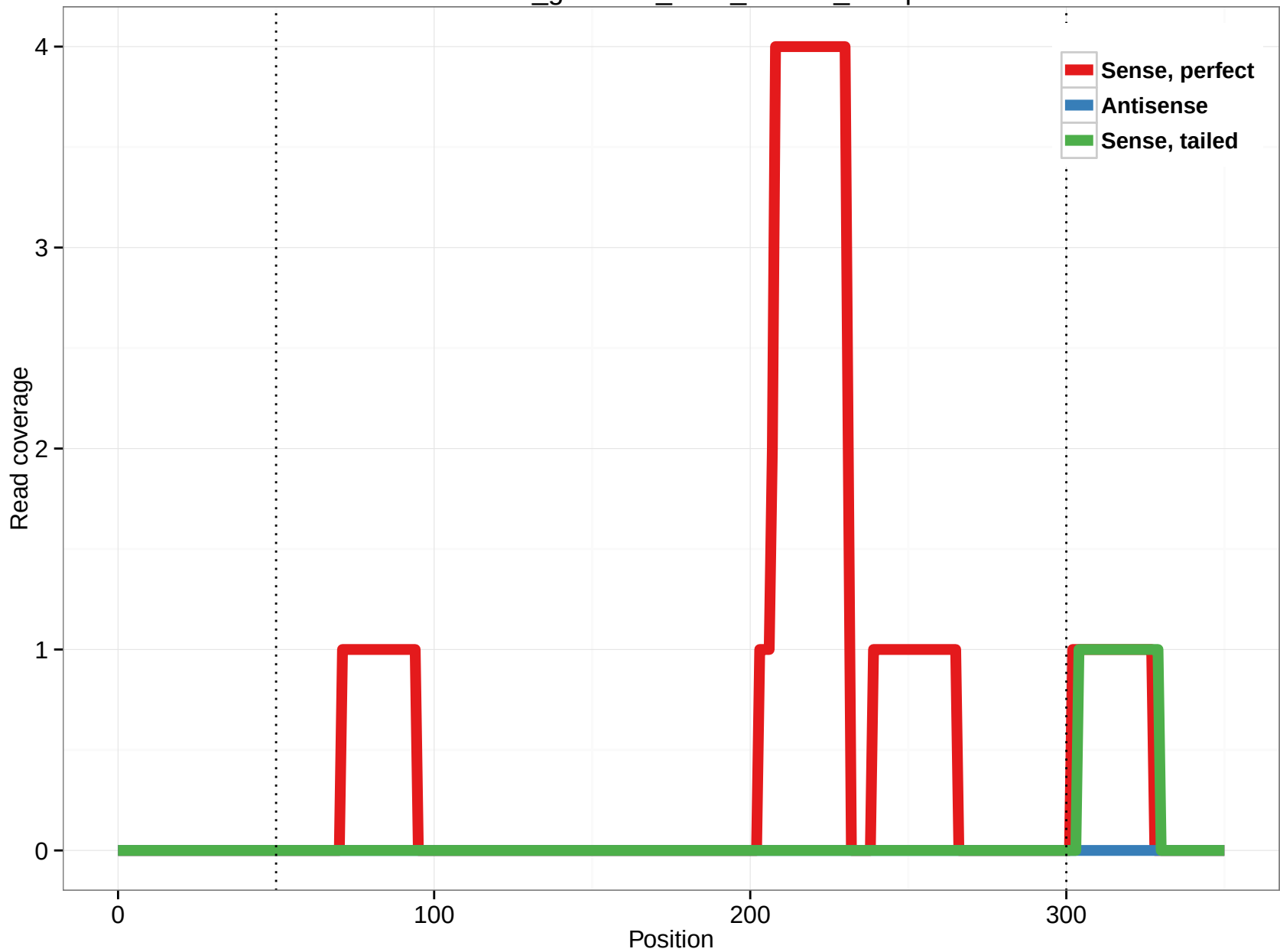
rheMac3_genscan_chrX_105.17_22.3p
