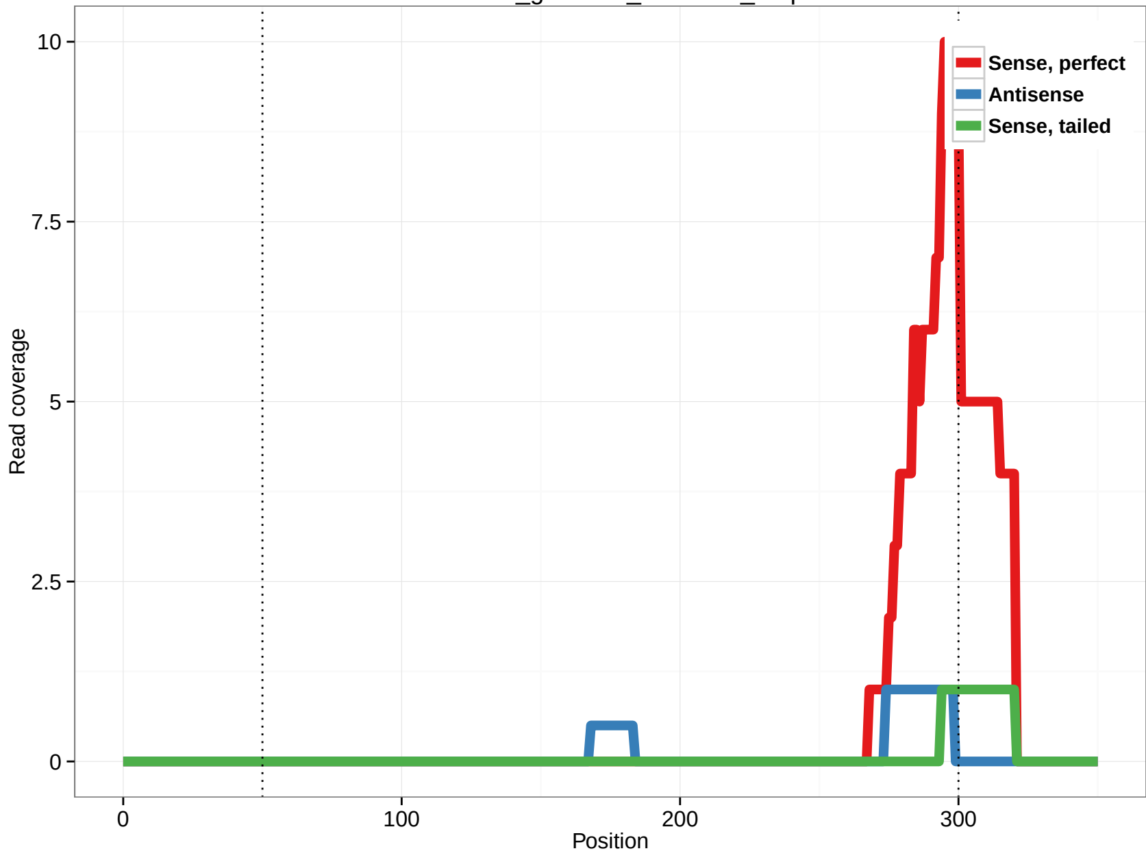
rheMac3_genscan_chr9.971_5.3p
