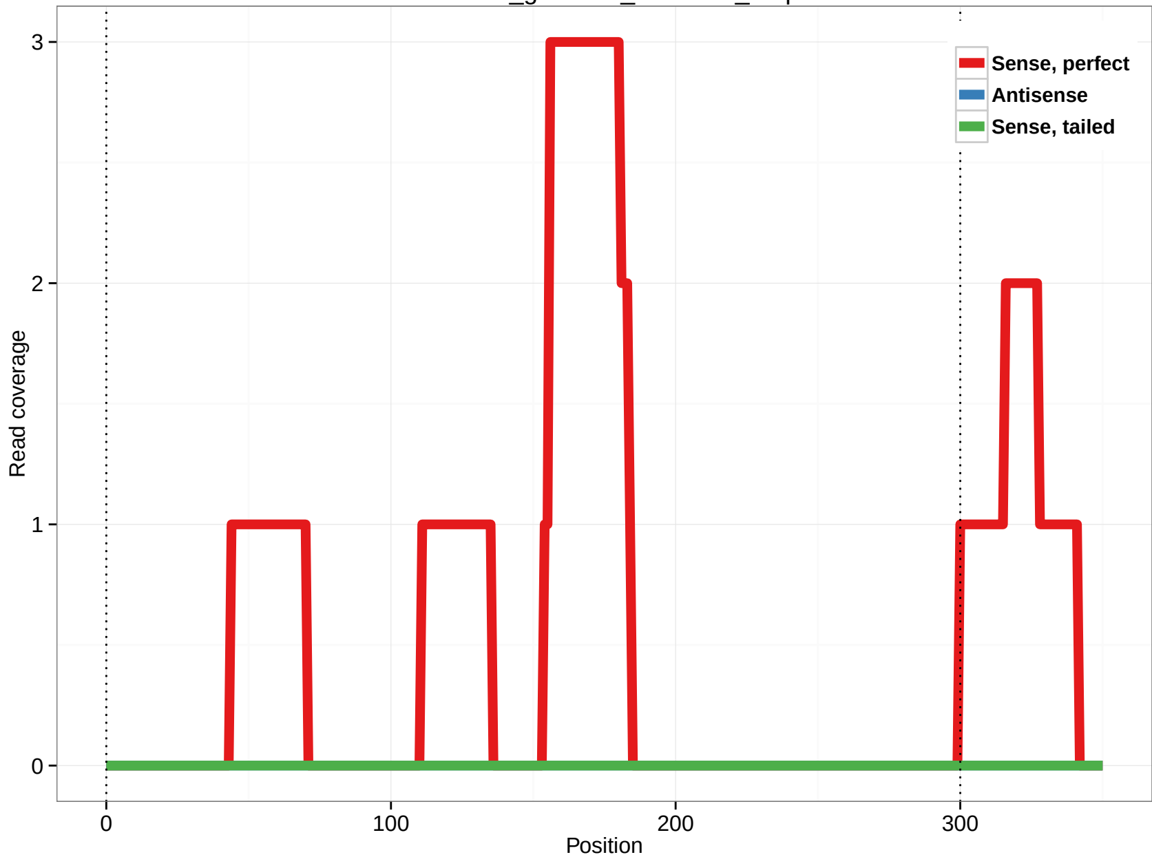
rheMac3_genscan_chr9.960_6.3p
