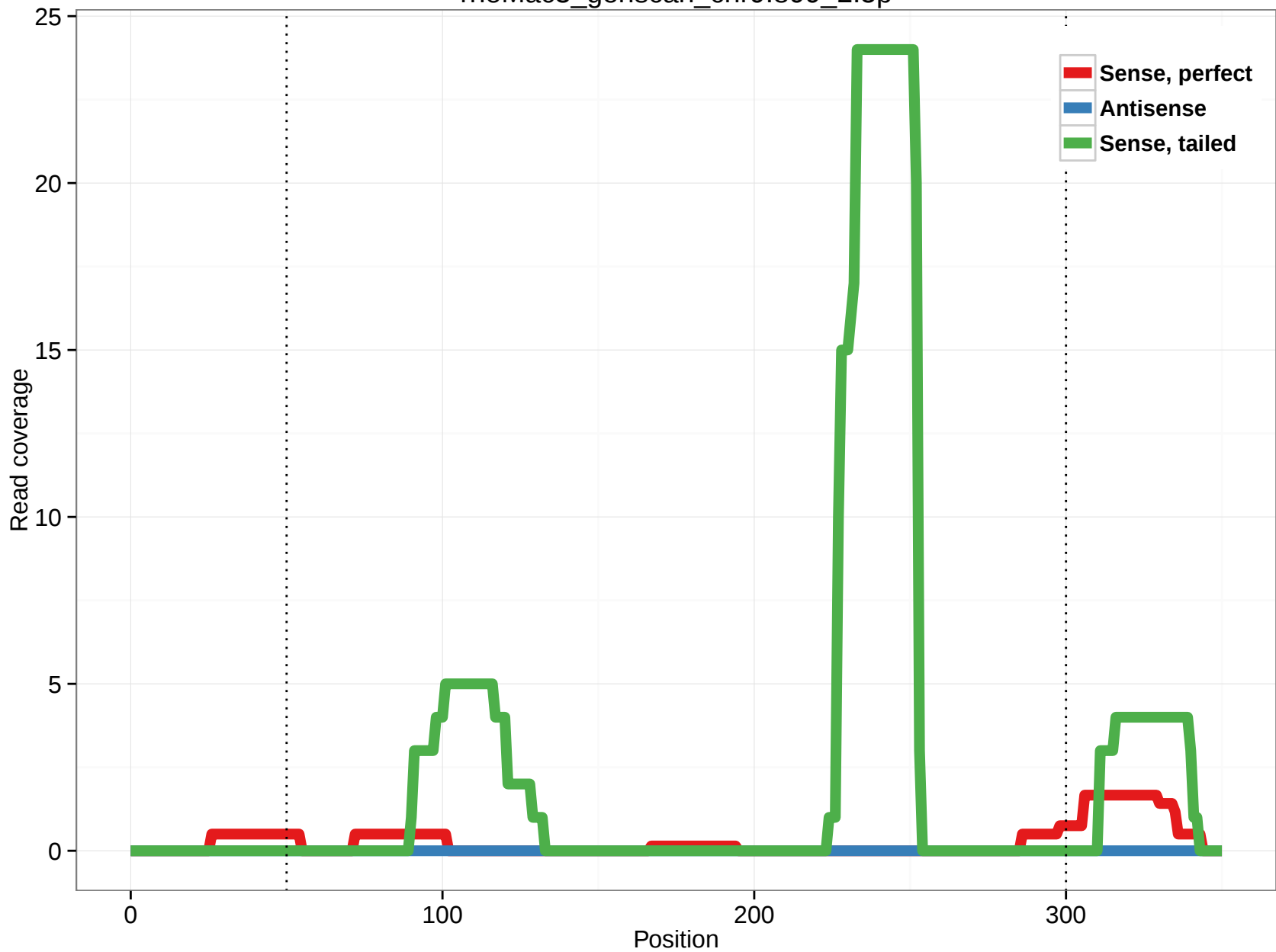
rheMac3_genscan_chr9.899_2.5p
