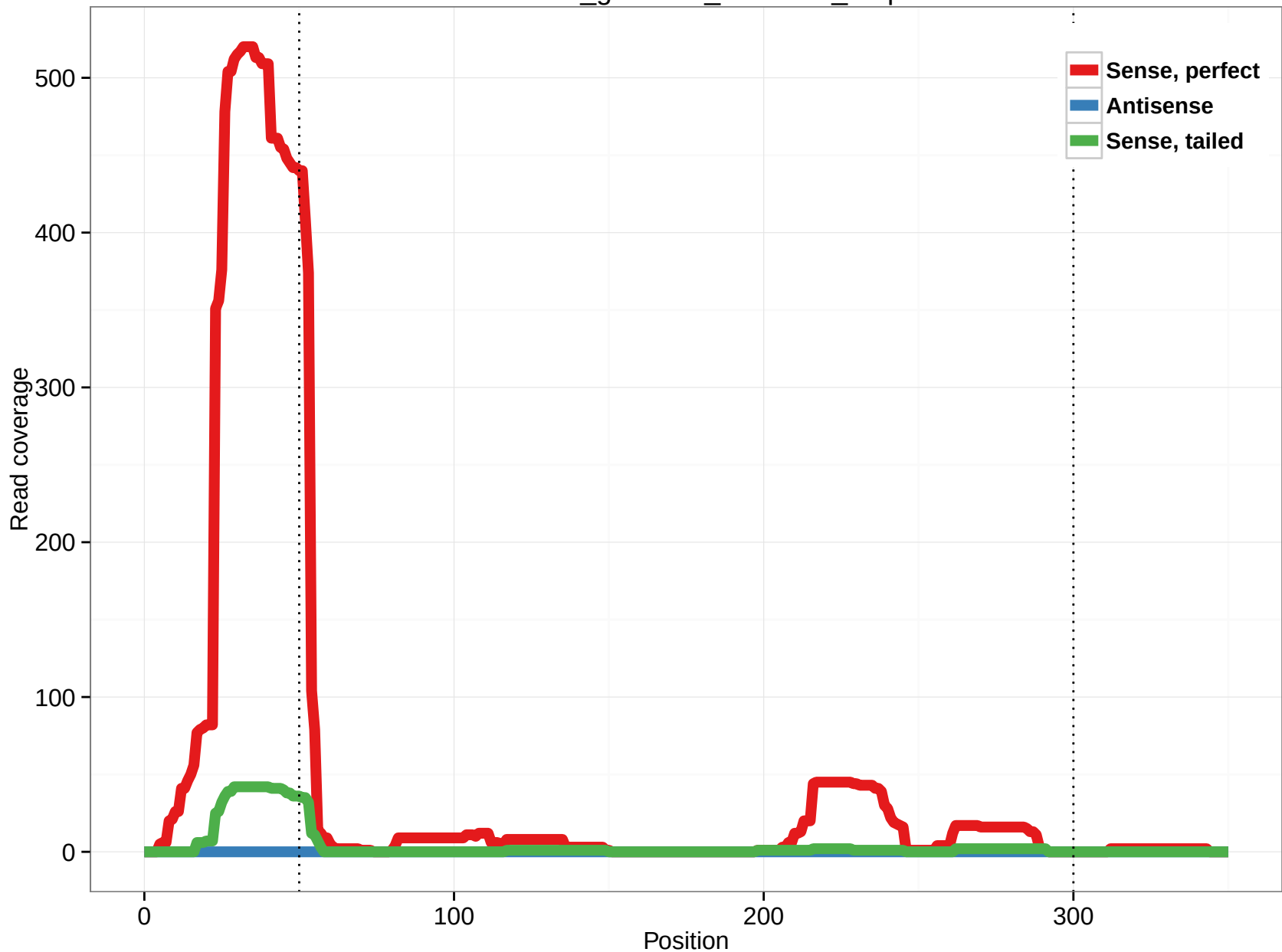
rheMac3_genscan_chr9.883_2.5p
