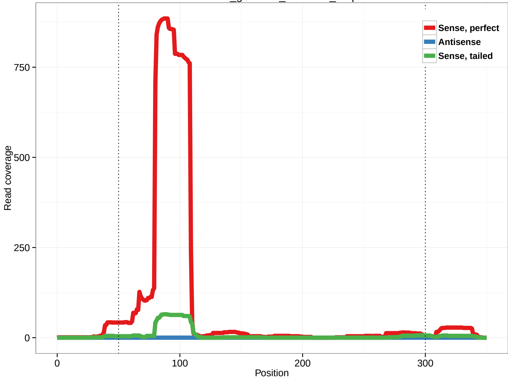
rheMac3_genscan_chr9.883_0.5p
