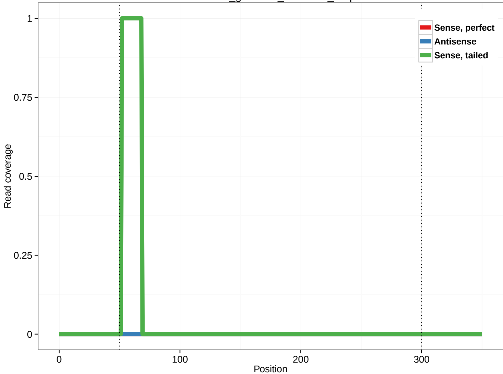
rheMac3_genscan_chr9.877_3.3p
