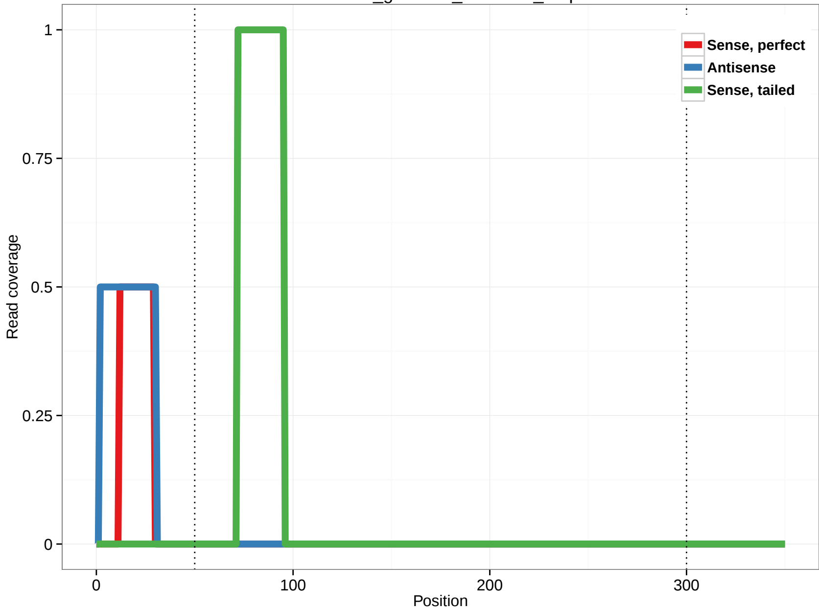
rheMac3_genscan_chr9.856_3.5p
