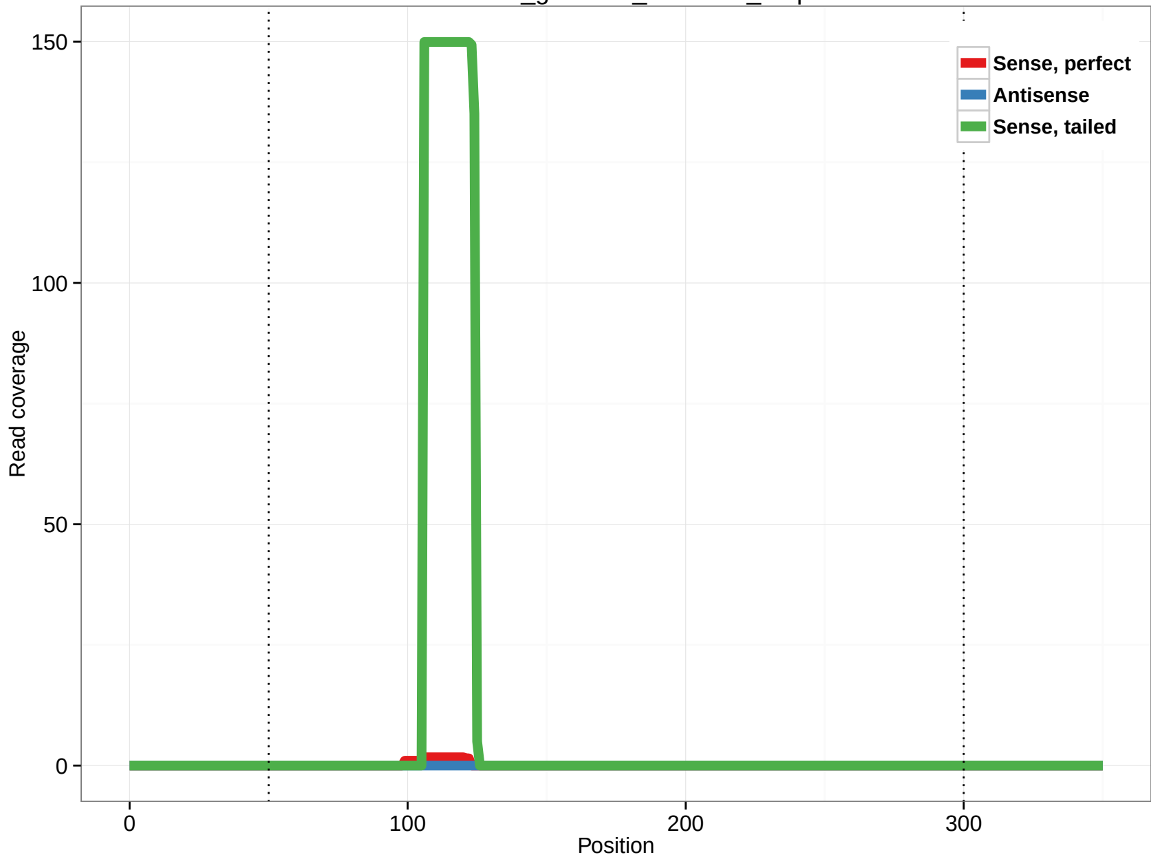
rheMac3_genscan_chr9.830_5.5p
