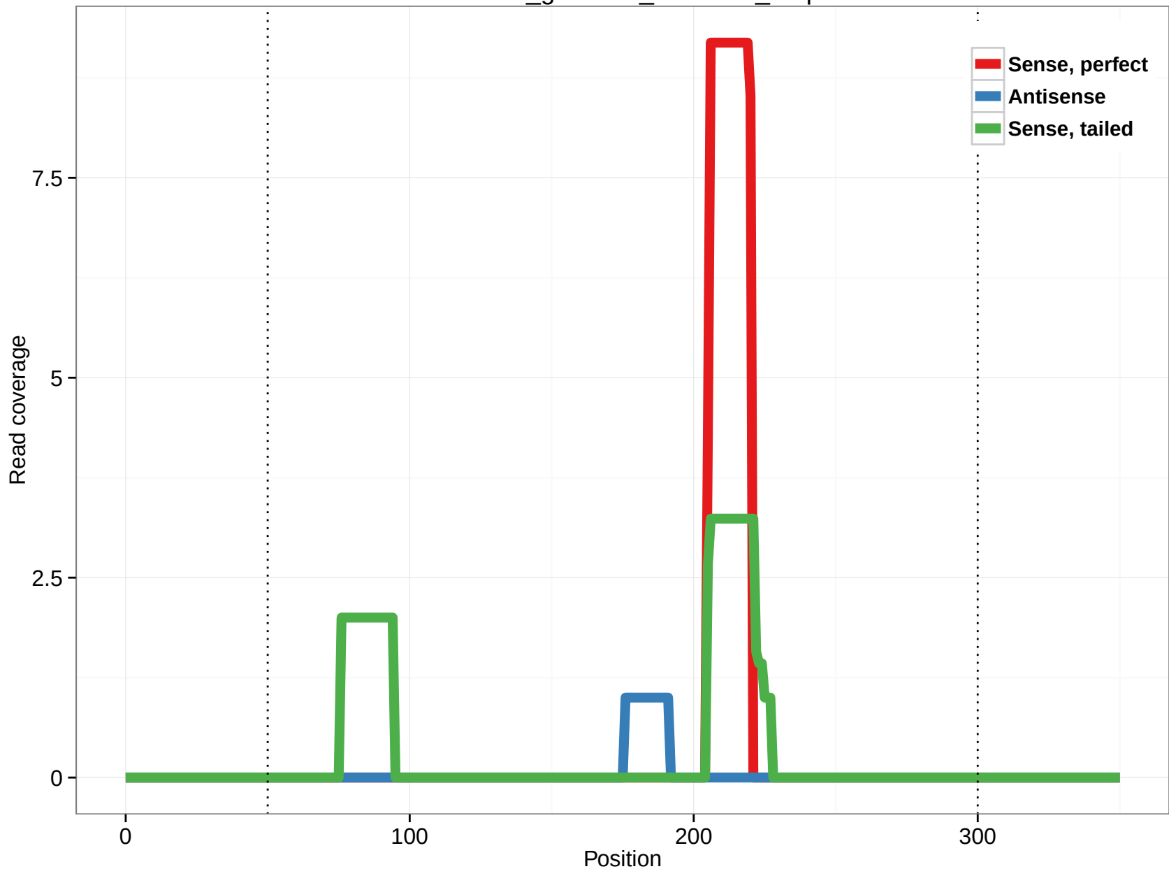
rheMac3_genscan_chr9.830_2.5p
