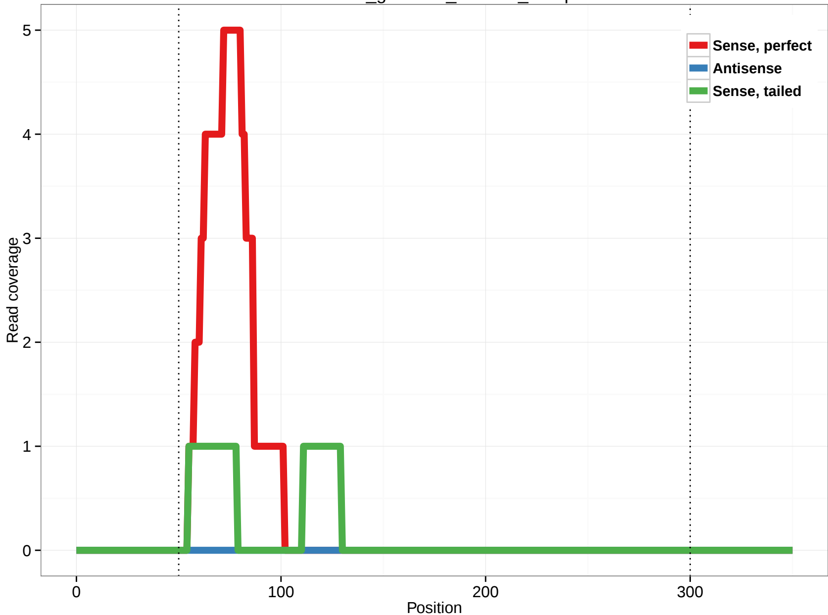
rheMac3_genscan_chr9.75_13.3p
