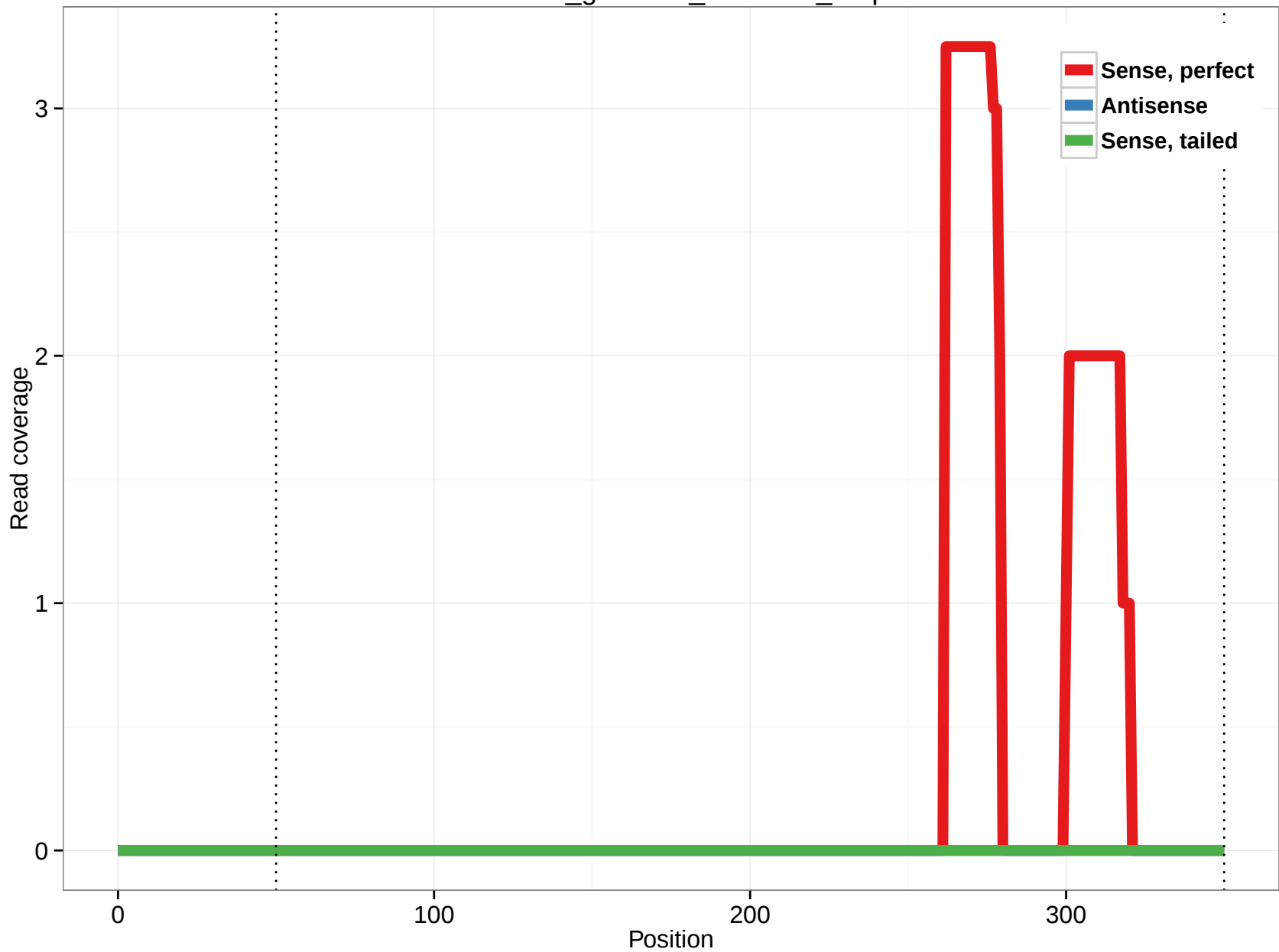
rheMac3_genscan_chr9.758_0.5p
