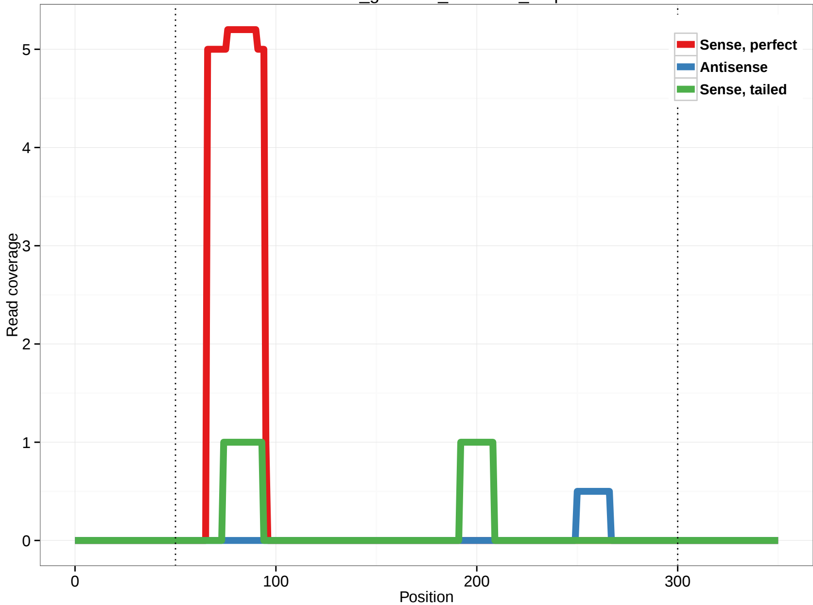
rheMac3_genscan_chr9.749_0.3p
