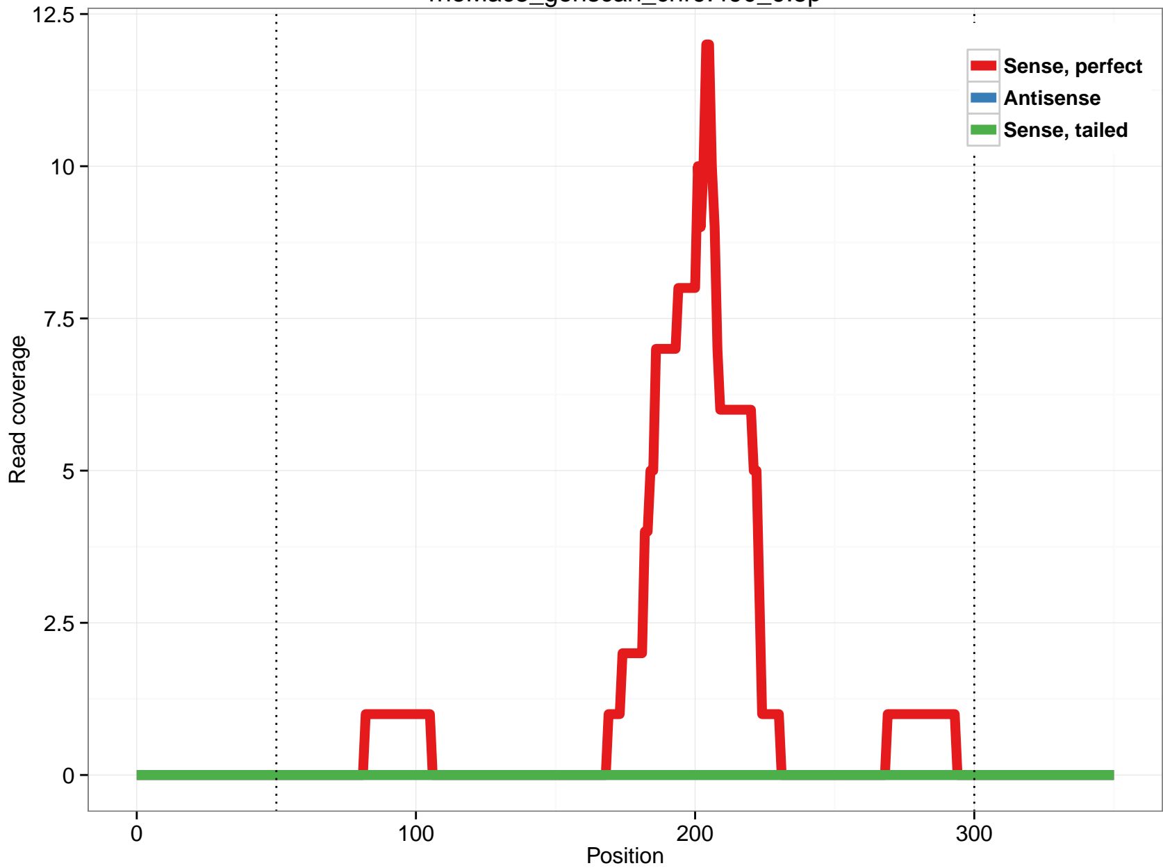
rheMac3_genscan_chr9.490_9.5p
