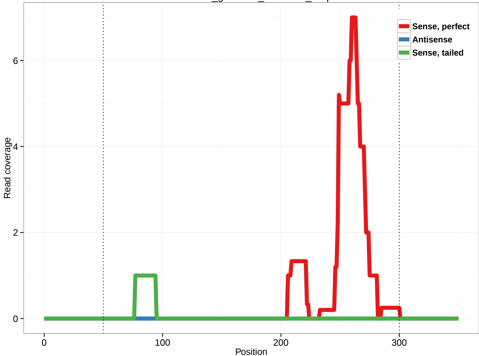
rheMac3_genscan_chr9.448_0.3p
