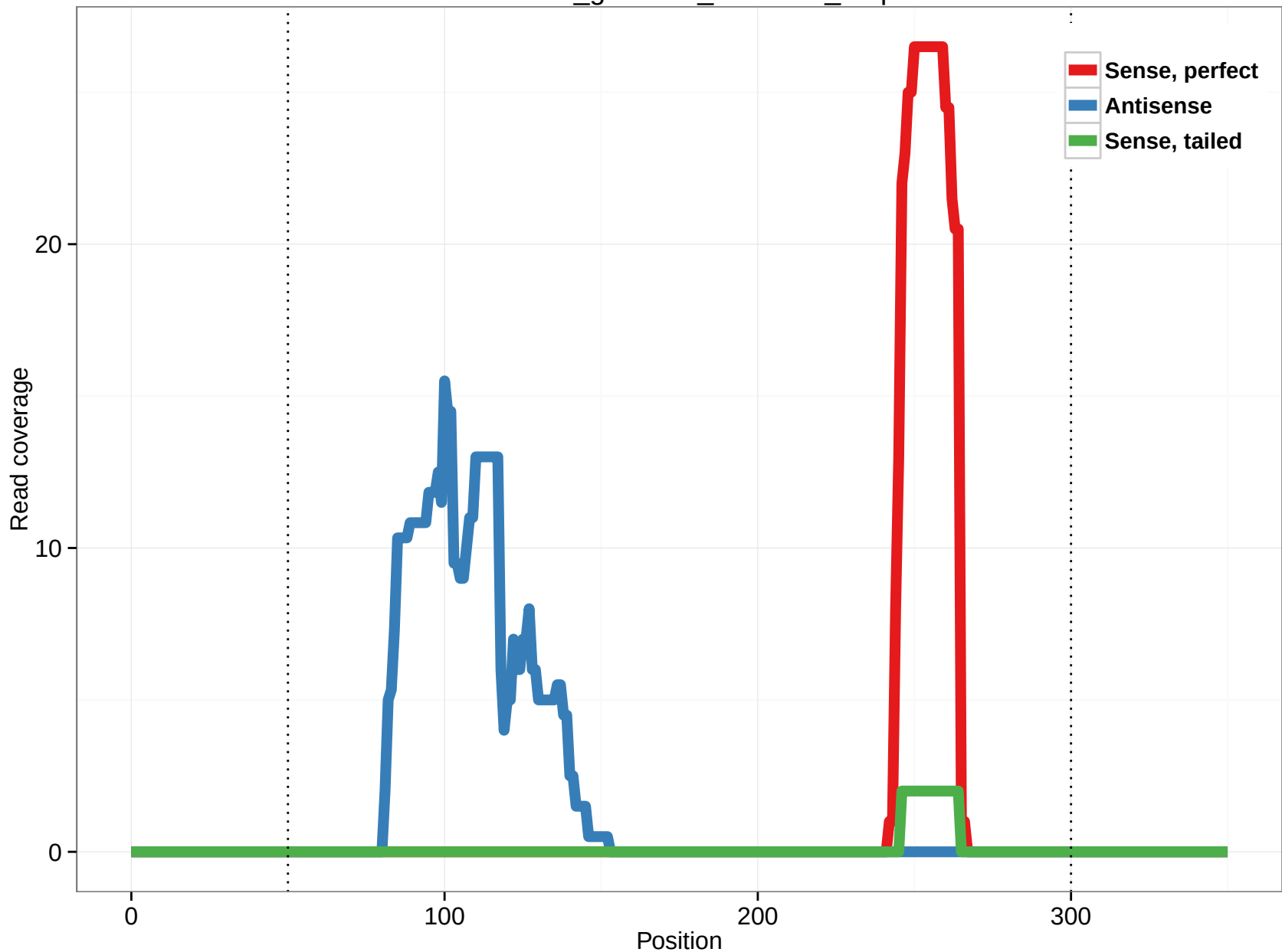
rheMac3_genscan_chr9.415_2.5p
