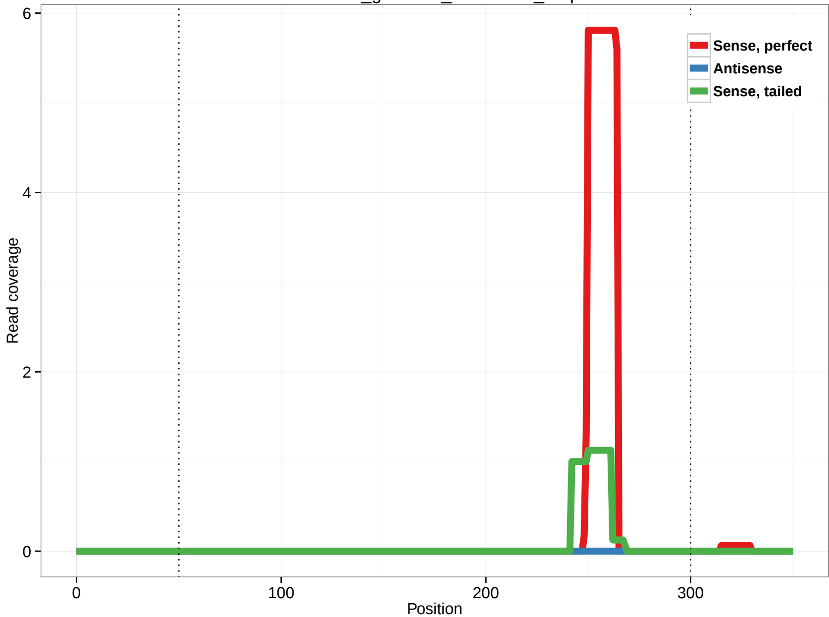
rheMac3_genscan_chr9.2750_8.5p
