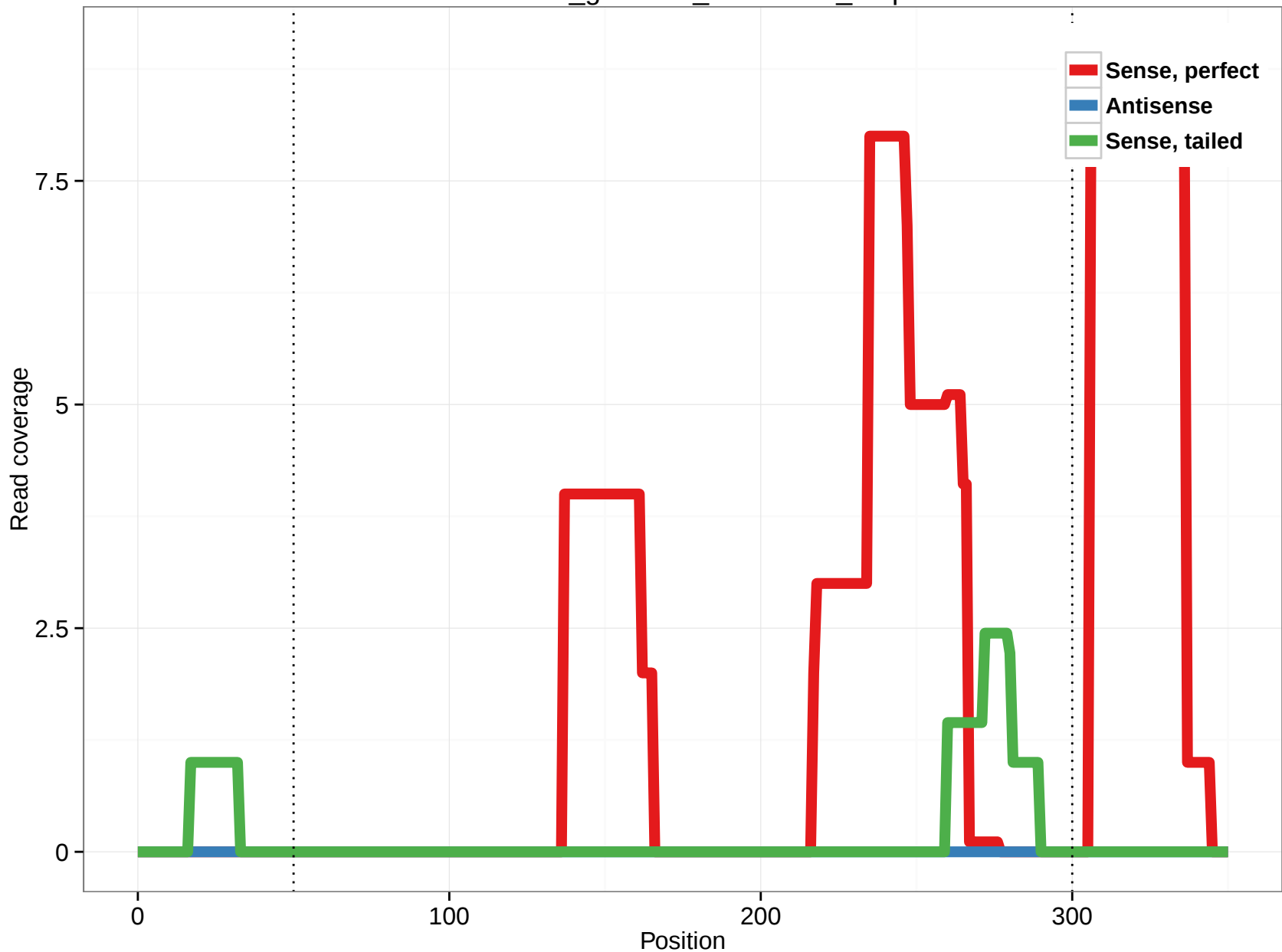
rheMac3_genscan_chr9.2690_1.5p
