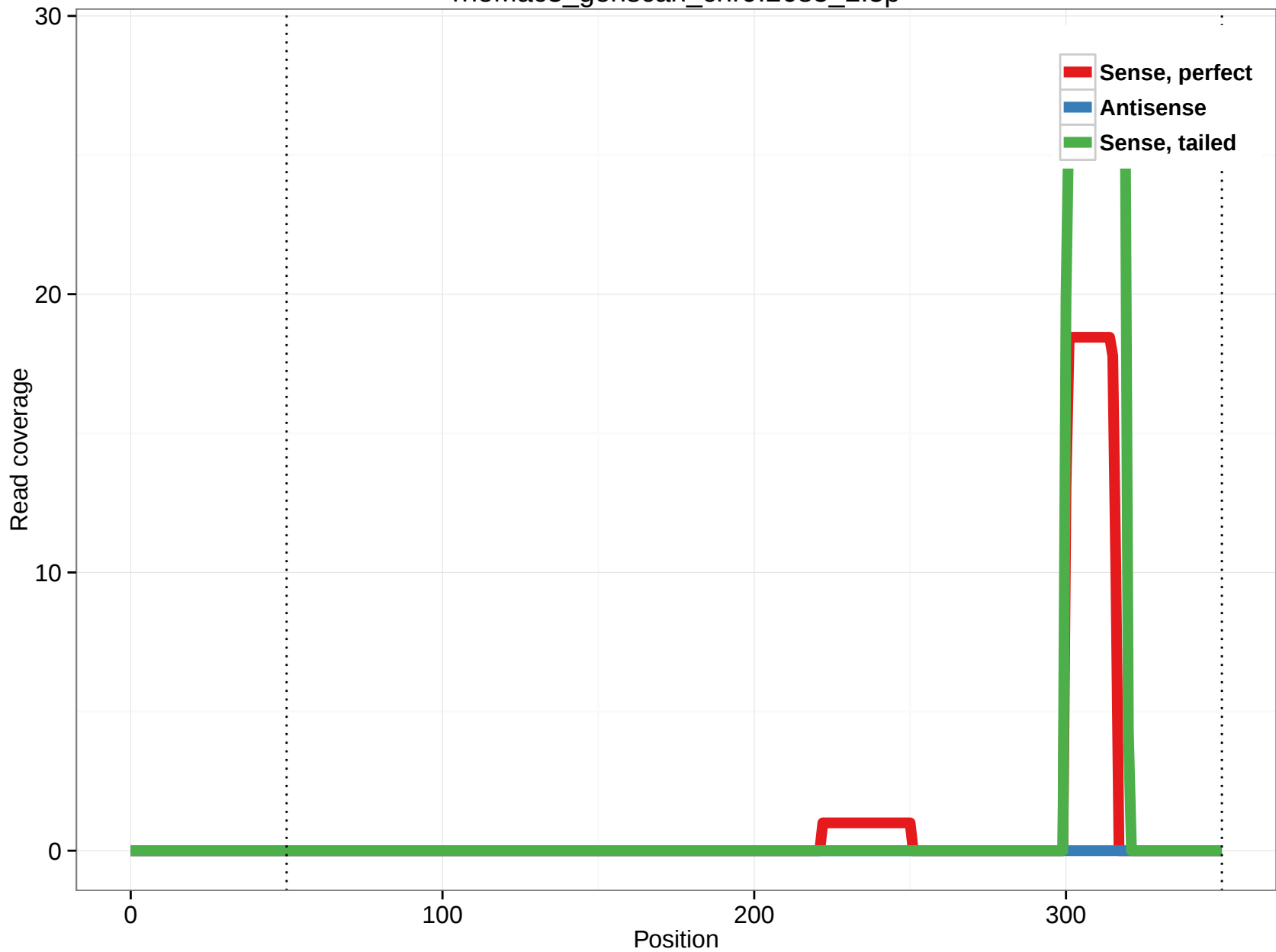
rheMac3_genscan_chr9.2685_2.5p
