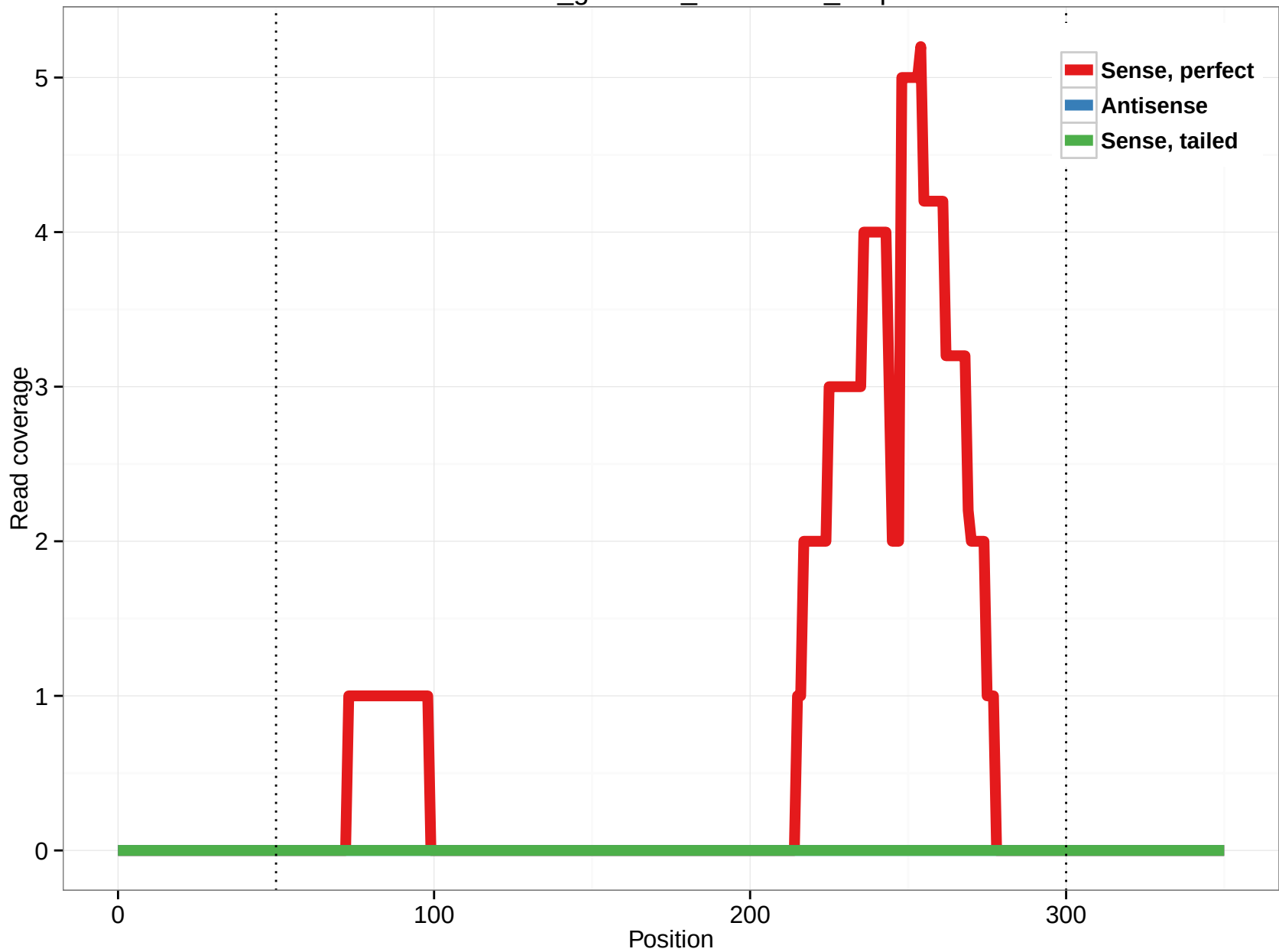
rheMac3_genscan_chr9.2566_8.3p
