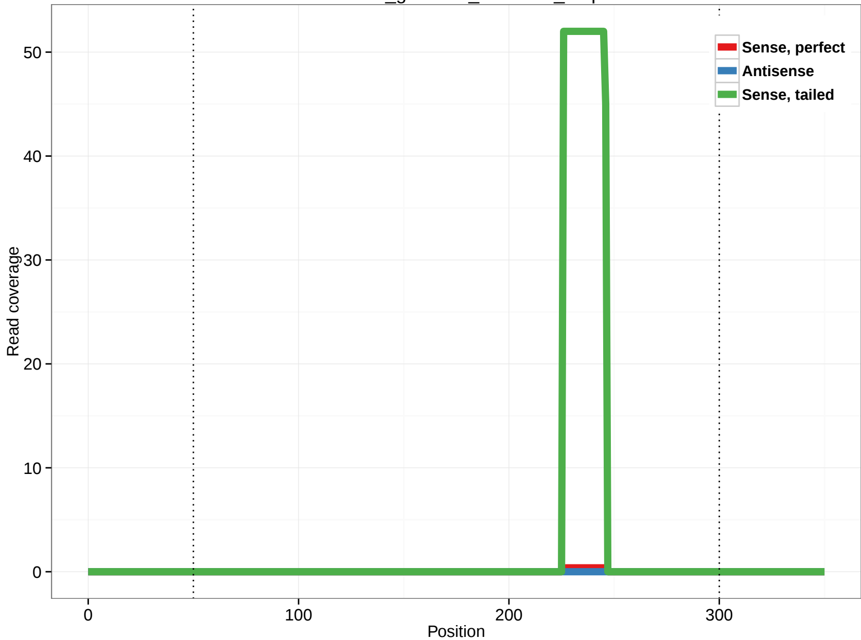
rheMac3_genscan_chr9.242_5.5p
