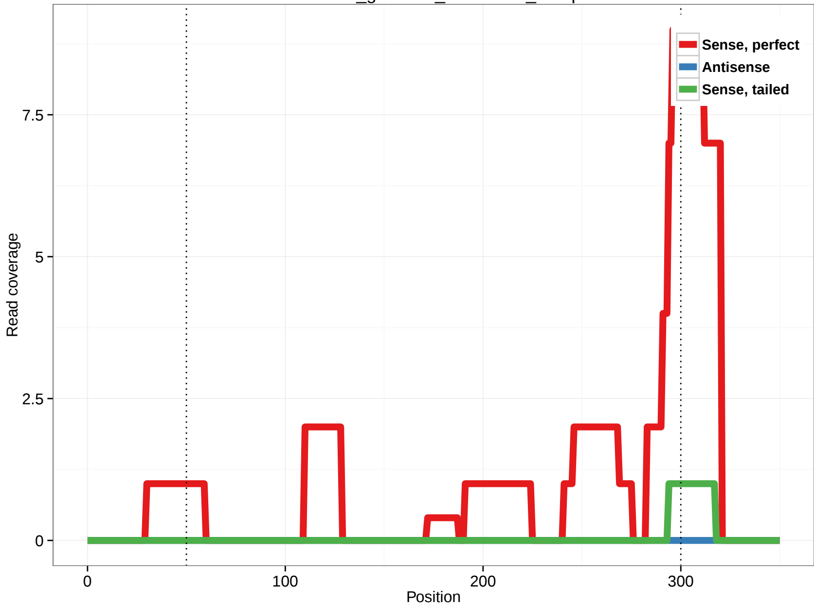
rheMac3_genscan_chr9.2421_27.5p
