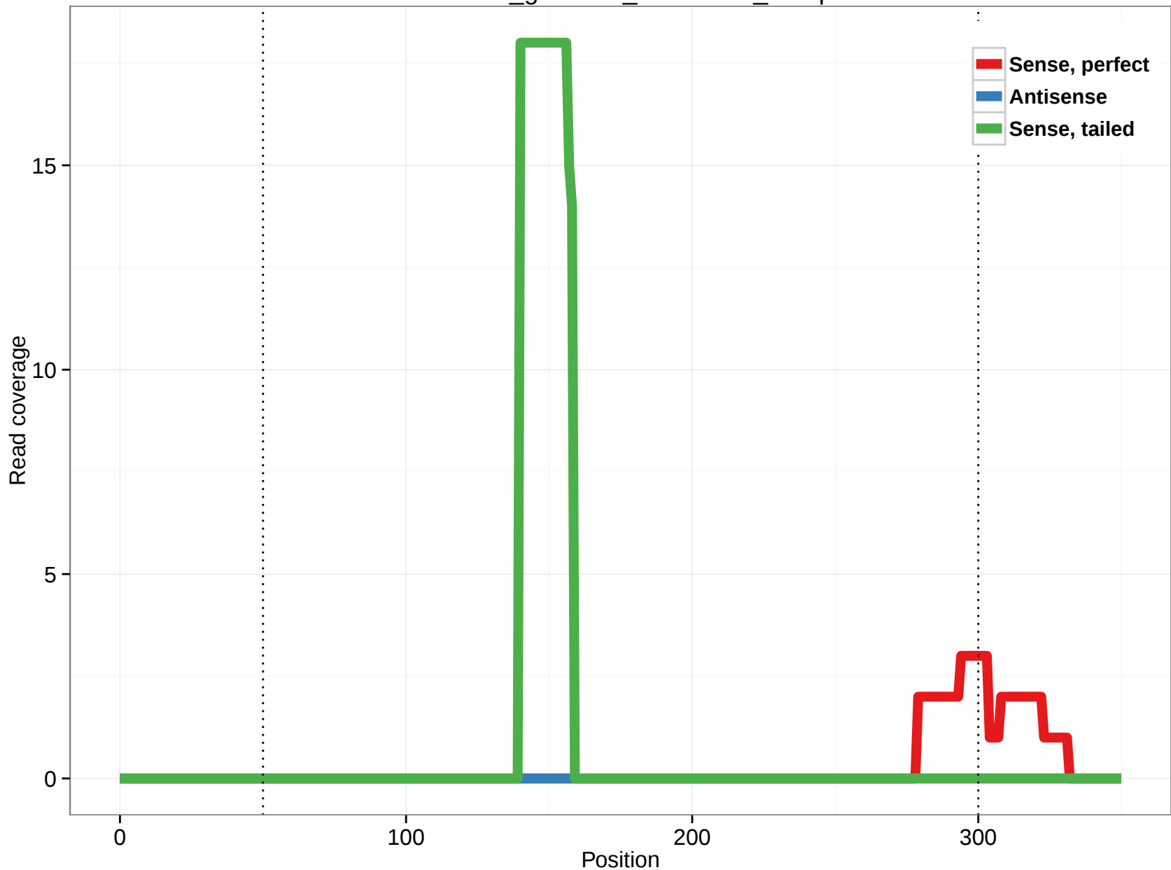
rheMac3_genscan_chr9.2408_44.3p
