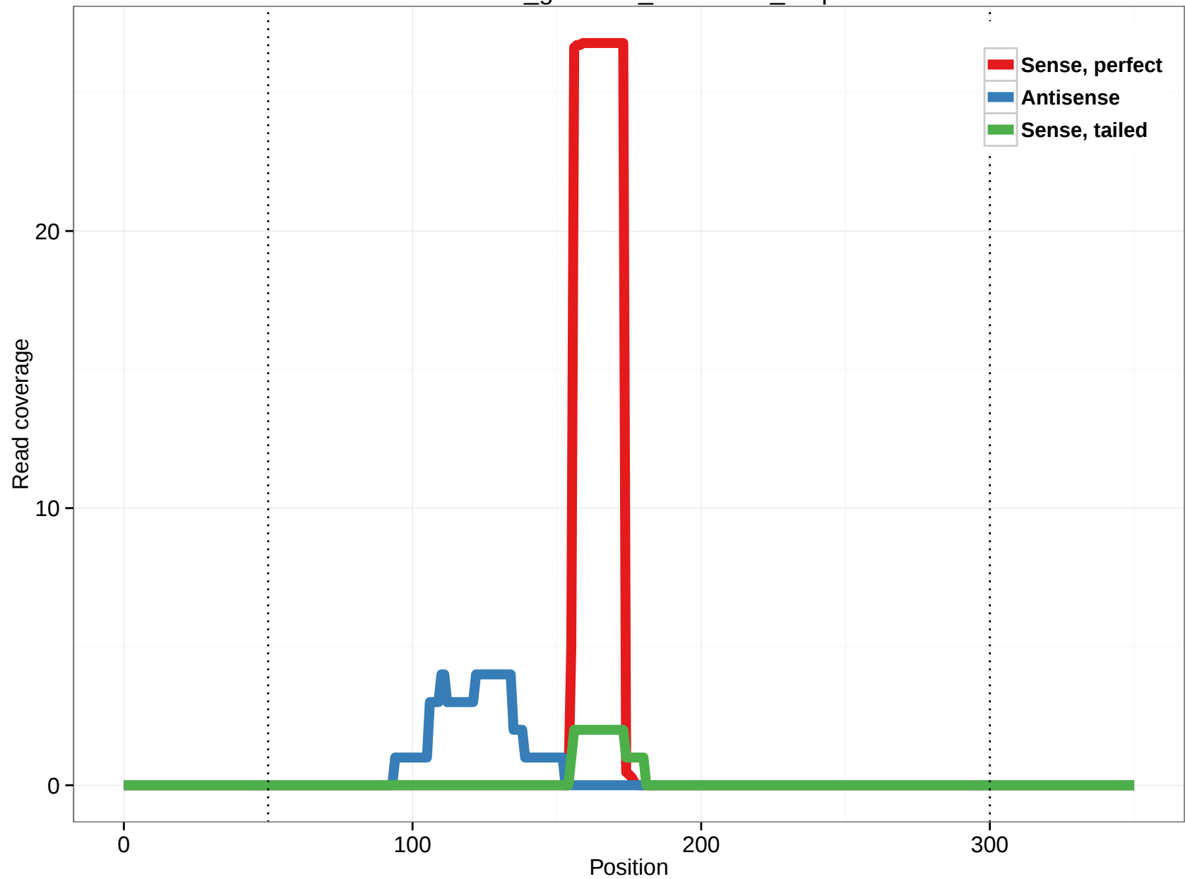
rheMac3_genscan_chr9.2376_0.3p
