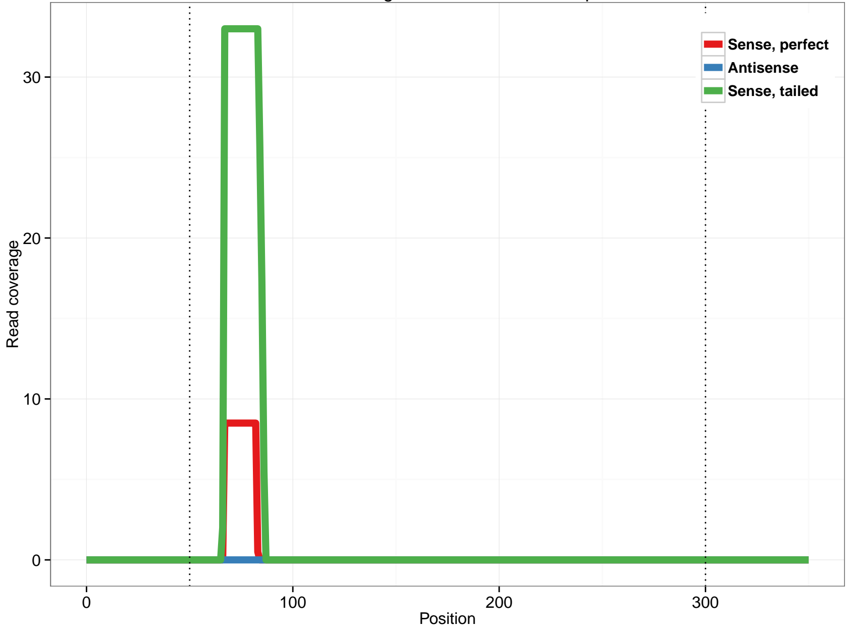
rheMac3_genscan_chr9.2270_2.5p
