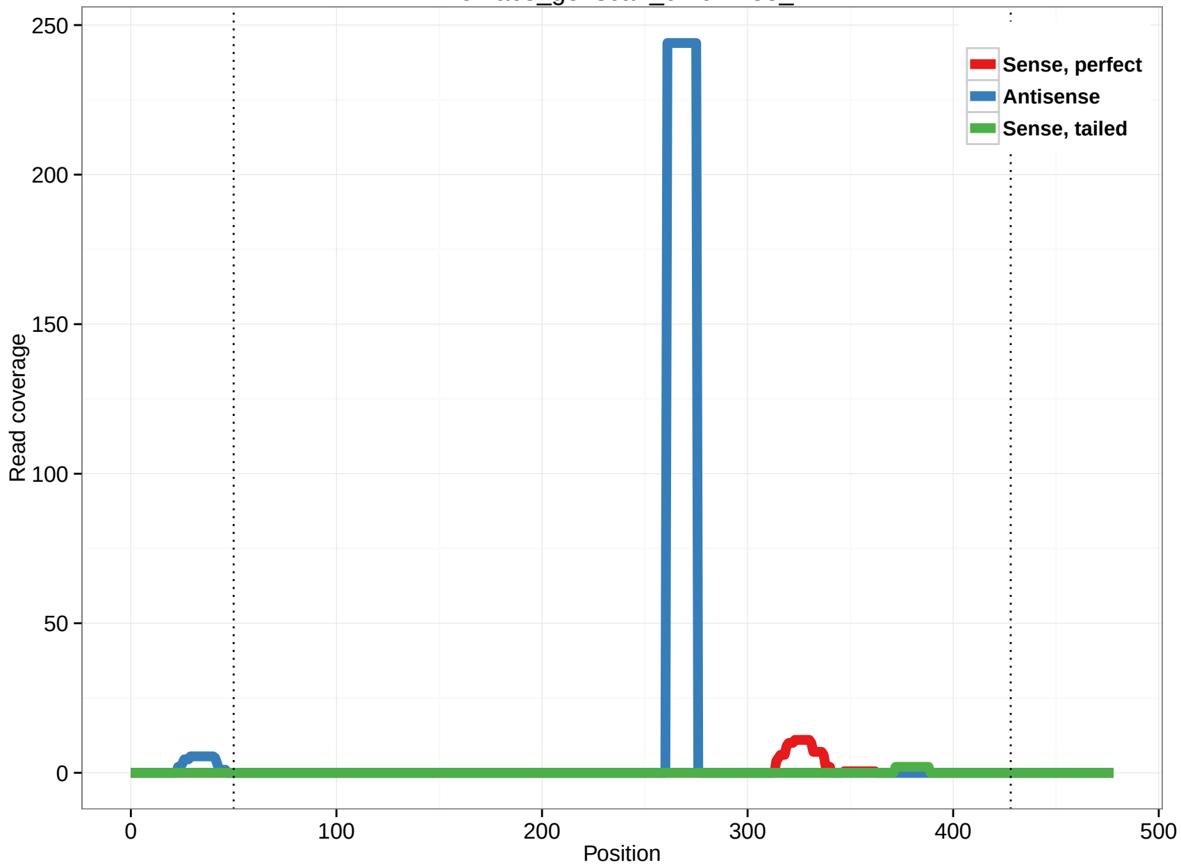
rheMac3_genscan_chr9.2233_2
