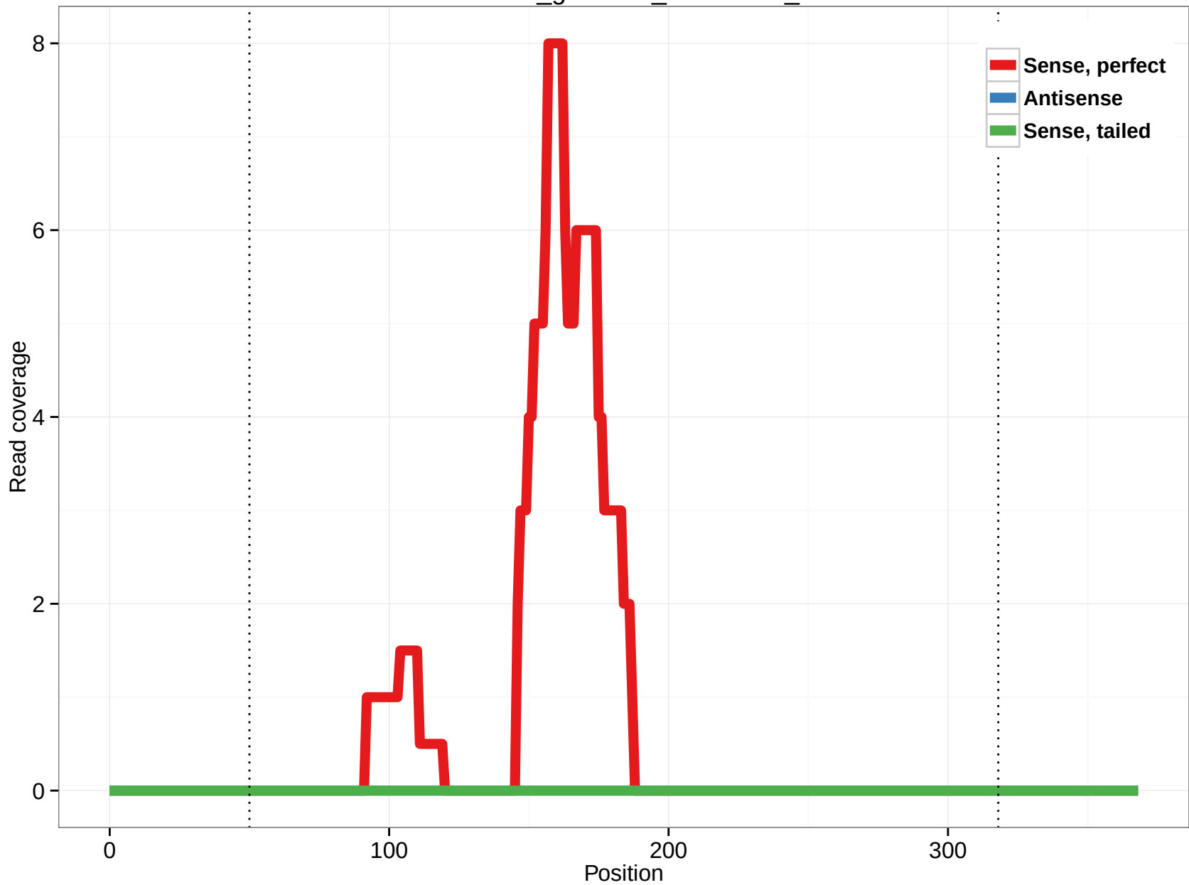
rheMac3_genscan_chr9.2163_4
