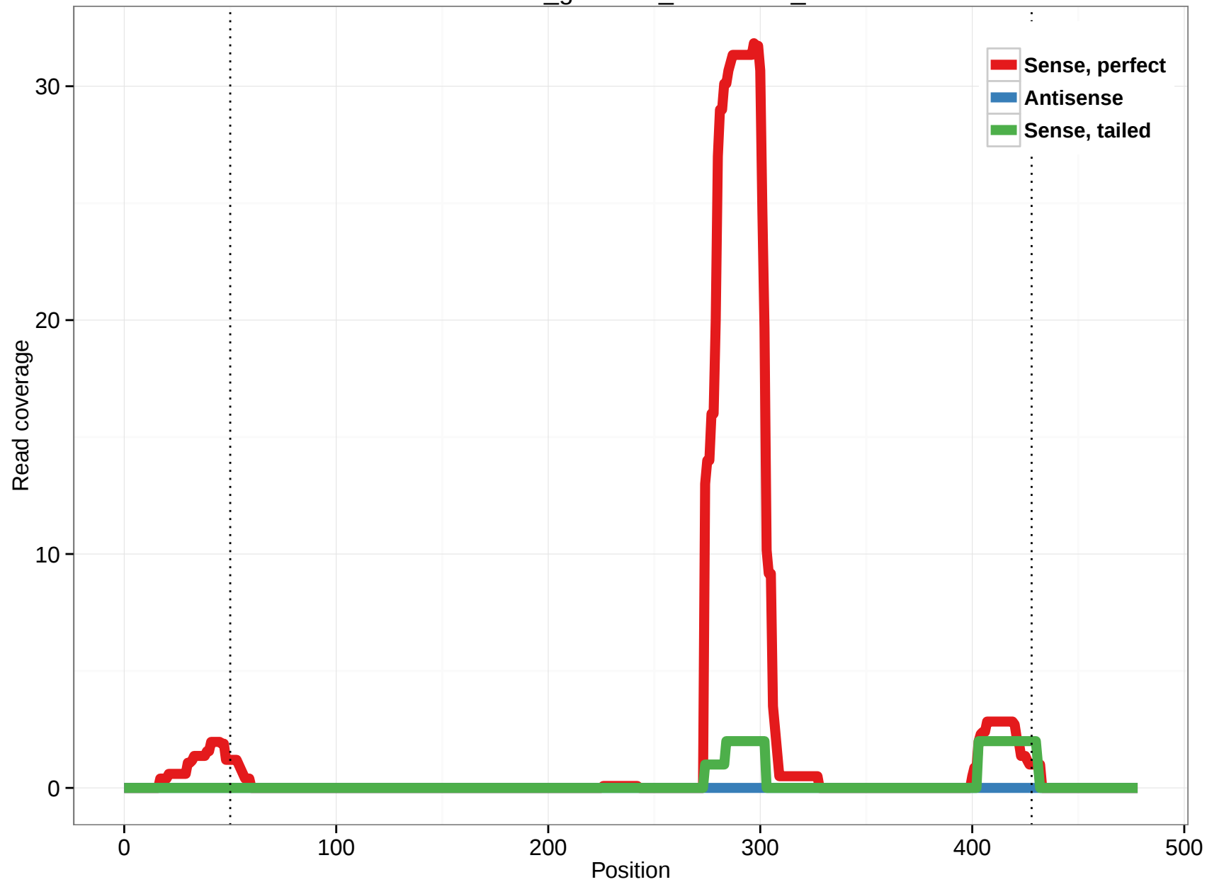
rheMac3_genscan_chr9.2102_2
