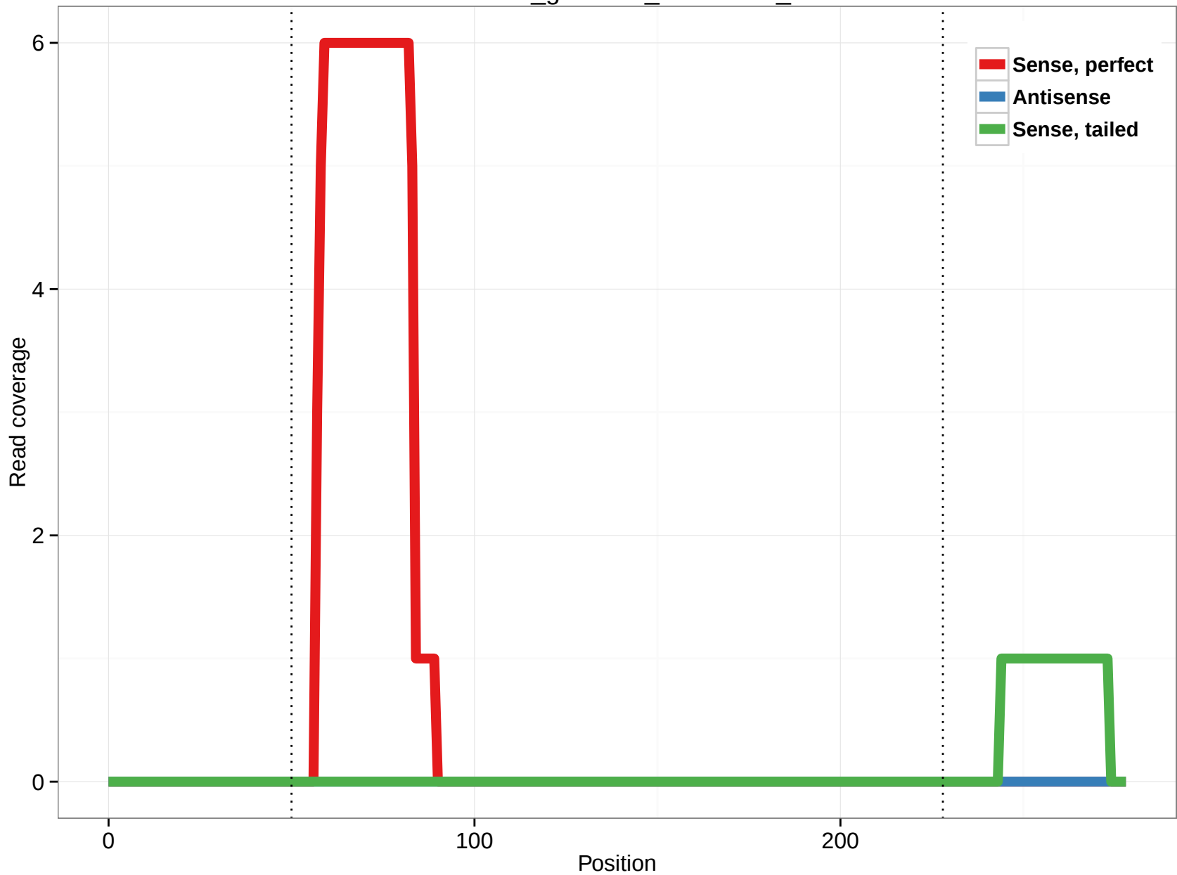
rheMac3_genscan_chr9.2076_1
