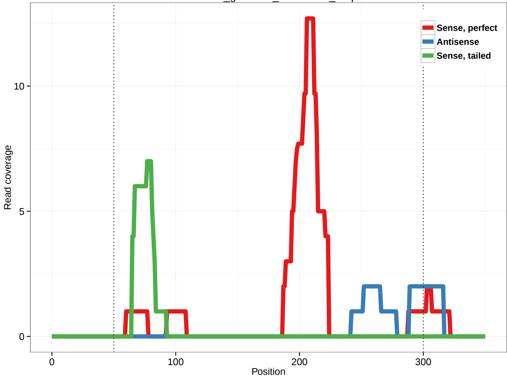
rheMac3_genscan_chr9.2072_0.3p
