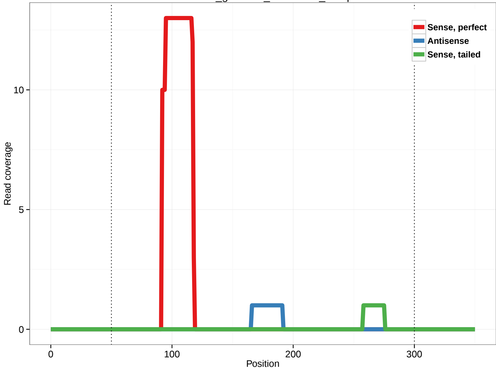
rheMac3_genscan_chr9.2051_21.5p
