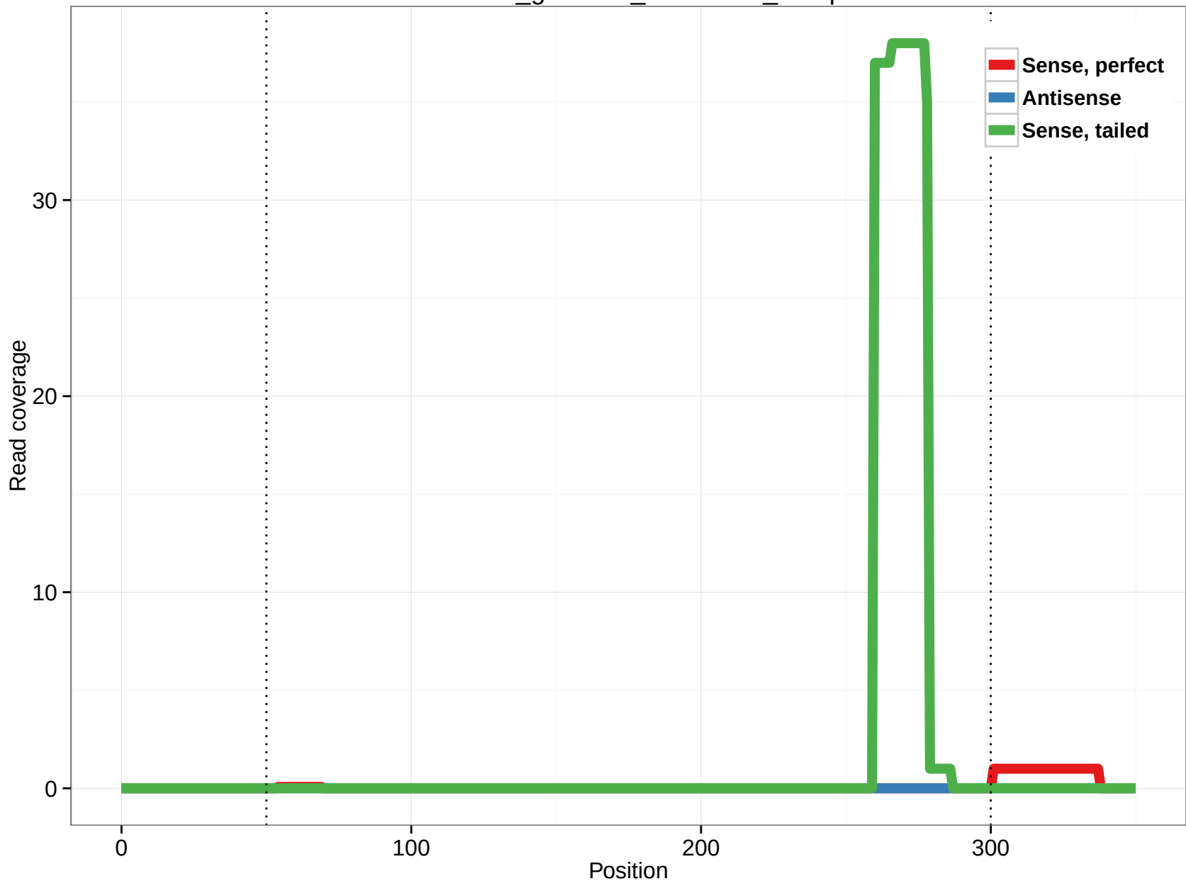
rheMac3_genscan_chr9.2051_15.3p
