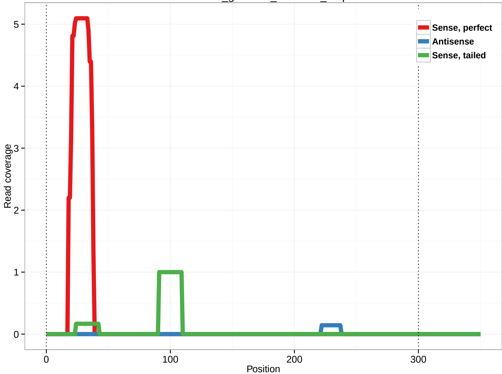
rheMac3_genscan_chr9.204_1.3p
