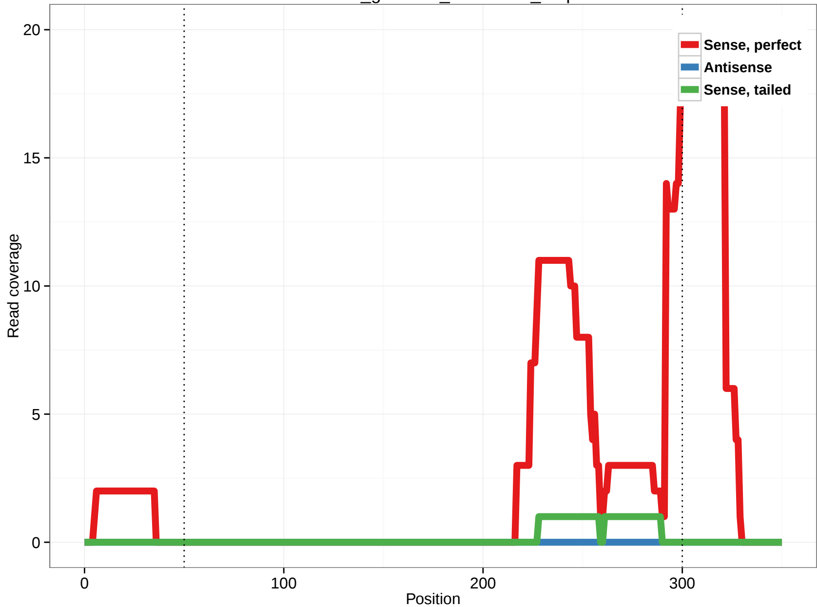
rheMac3_genscan_chr9.1995_3.3p
